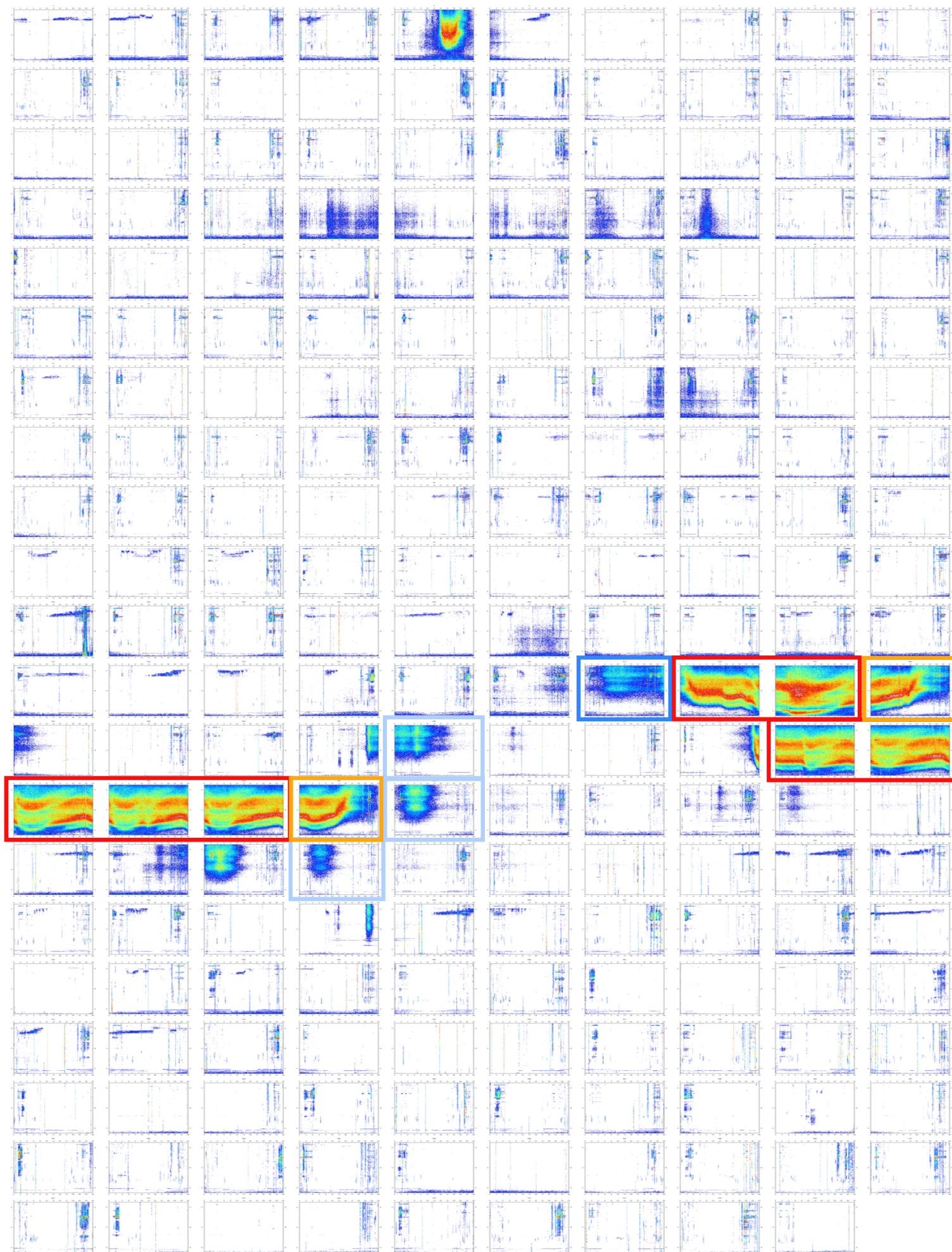
Supplemental Figure S2: Daily spectrograms for year 2012 (Julian days 1-200). Each spectrogram begins at 12:00 UTC and end at the same hour the next day. Frequency range: 1.5 - 6.5 Hz. Color boxes show the results from the hierarchical classification (see Fig 8).
