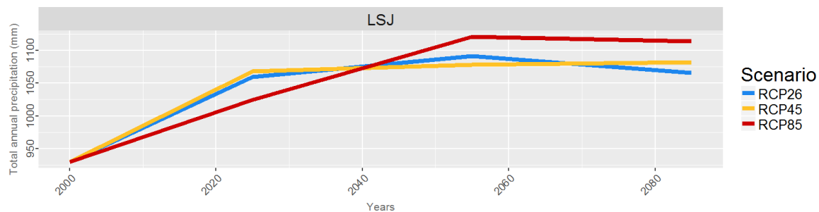
S1 Fig. Current and future projections for a) mean annual temperature (MAT) and b) total annual precipitation from the Canadian Coupled Global Climate Model CanESM2 for each of the three different forcing scenarios i.e. RCP 2.6, RCP 4.5 and RCP 8.5 used in our simulations. Baseline (1981-2010) and future 30-year values were averaged to better reflect the climate data that were used in LANDIS-II to parameterize tree growth.
