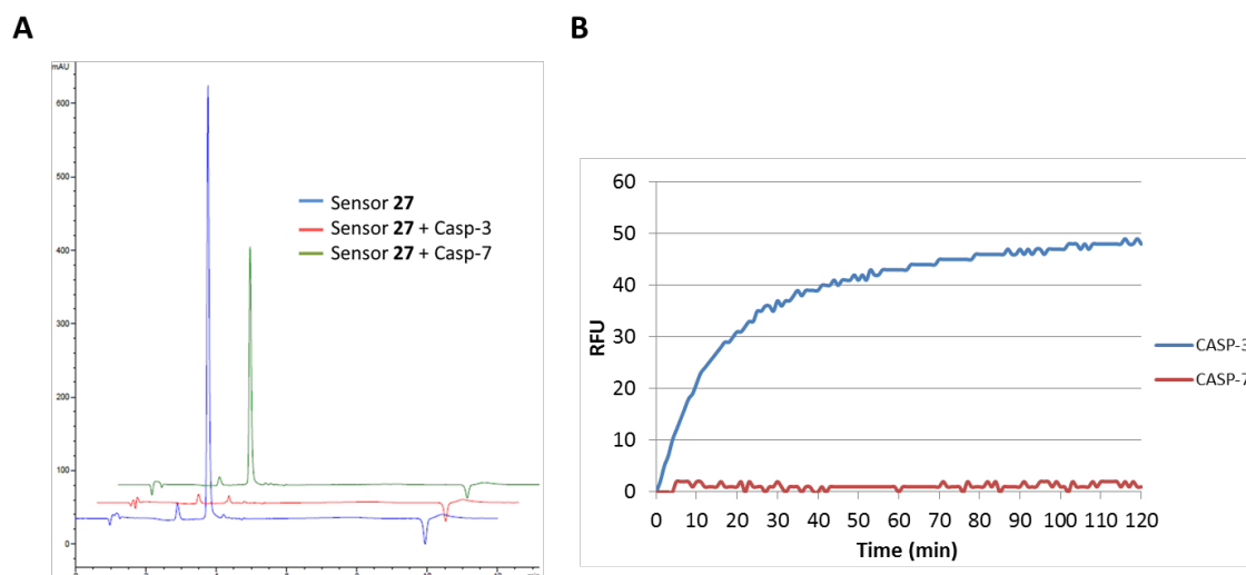
S7 Fig. (A) HPLC chromatogram (detection at 254 nm) of substrate 27 (10 \mu M) after 120 min incubation with caspase-3 or caspase-7 (0.3 \mu M). (B) Time-dependent increase in fluorescence ( \lambda_{\text{Ex/Em}} 485/528 nm) of 27 (0.6 \mu M) during 120 min incubation with caspase-3 or -7 (15 nM).
