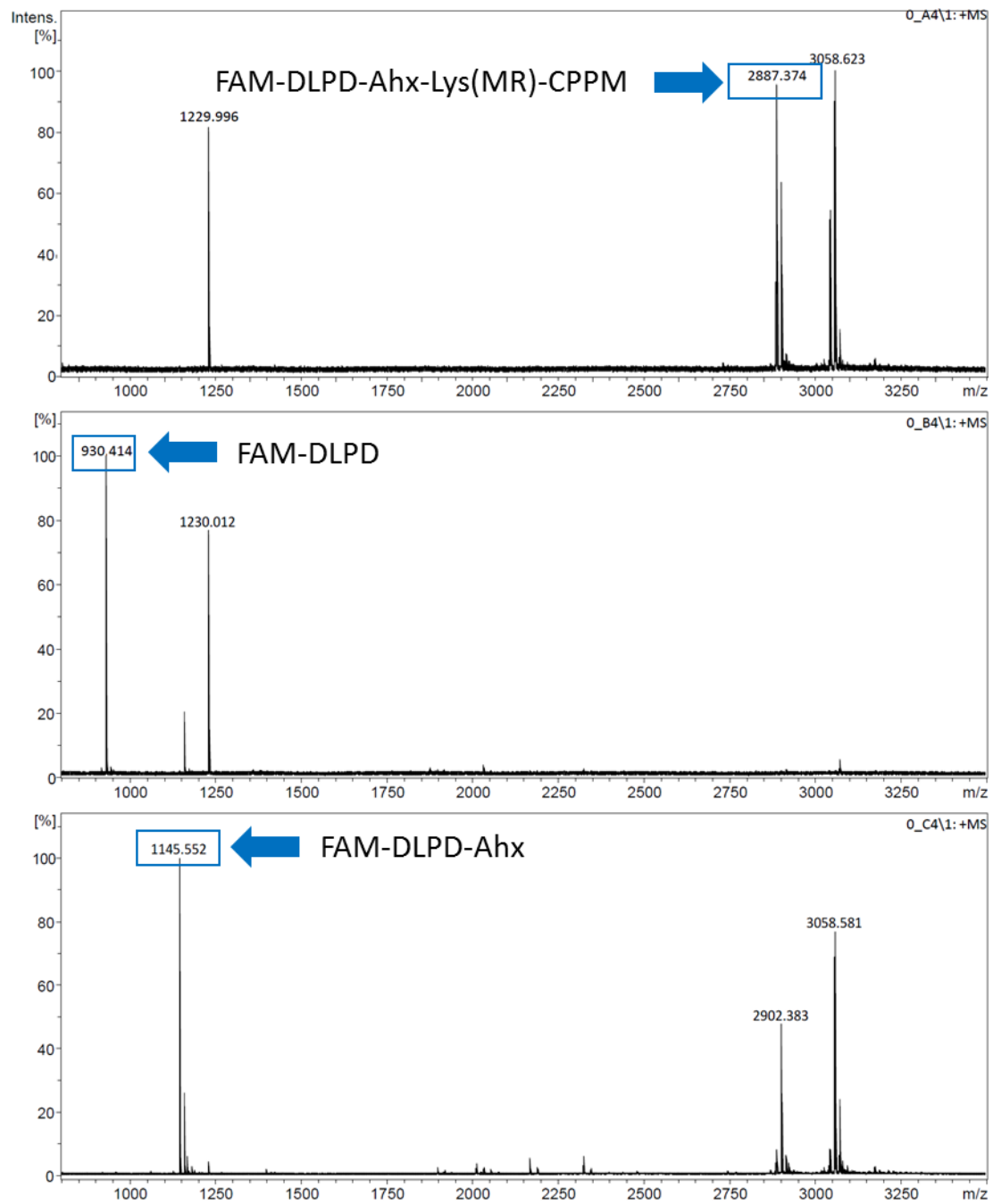
S3 Fig. A) MALDI-TOF MS spectra of substrate 12 (sequence Asp-Leu-Pro-Asp). (B) After incubation (20 \mu M) with Caspase-3 for 2 h. (C) After incubation (20 \mu M) with Caspase-7 for 2 h (detected as the PBS adduct.)
