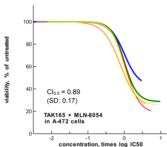
Supplementary Figure S8. Curve shift experiment of the combination of MLN-8054 (green) and TAK-165 (blue). Mixture ratios used were 1:1, red; 4:1, orange; 1:4, yellow. CI values and standard deviations (SD) are based on three mixtures (see Table S4 for individual values)
