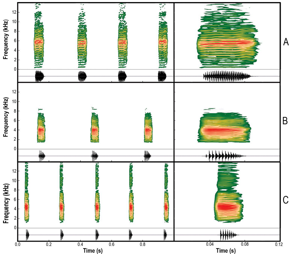
Fig 8. Audiospectrograms (above) and oscillograms (bellow) of the advertisement calls. (A) Scinax fontanarrosai sp. n. (LGE 4451), (B) S. pinima (UFMG 20184), and (C) S. uruguayus (MNHN 9877). Left: A series of calls. Right: A single call.
