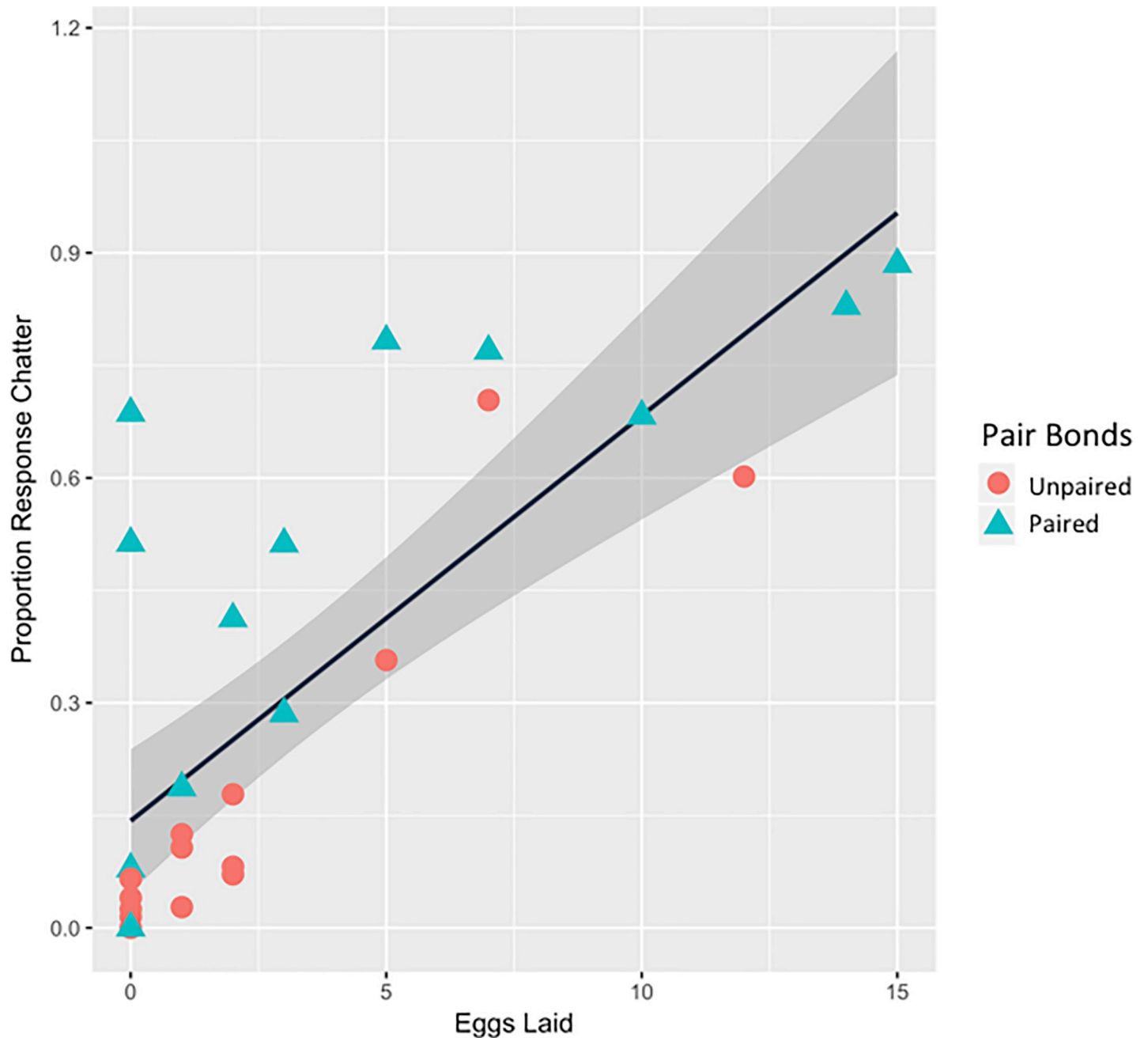
Fig 2. Relationship between proportion response chatters and eggs laid. Scatterplot for the proportion of response chatters and the number of eggs laid for all females. Females who formed a pair bond during 2012 season are shown as a triangle, and females who did not maintain a pair bond are shown as a circle. Line represents the permuted linear regression with surrounding 95% confidence intervals.
