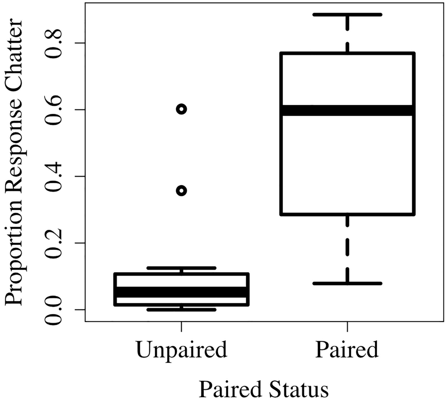
Fig 1. Proportion response chatters by paired status. The proportion of response chatter vocalizations based on an individual's paired status. Boxes represent interquartile ranges with the median in the middle represented by a bold line; whiskers represent the range of the highest and lowest values that are within a range of 1.5 times the interquartile range; dots indicate data points that are outside this range.
