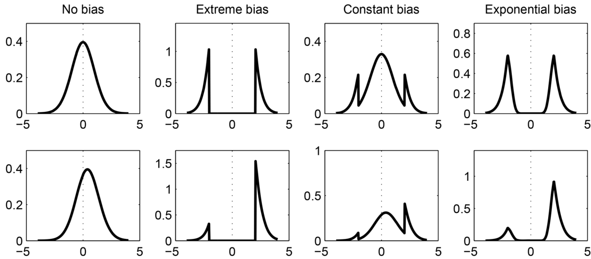
Fig 1. Predicted distributions of t statistics in the literature. Predicted distributions are shown under the four censoring mechanisms we consider (columns) and two possible states of nature (top row: \mathcal{H}_0 true ( \delta = 0 ); bottom row: \mathcal{H}_0 false ( \delta \neq 0 )).
