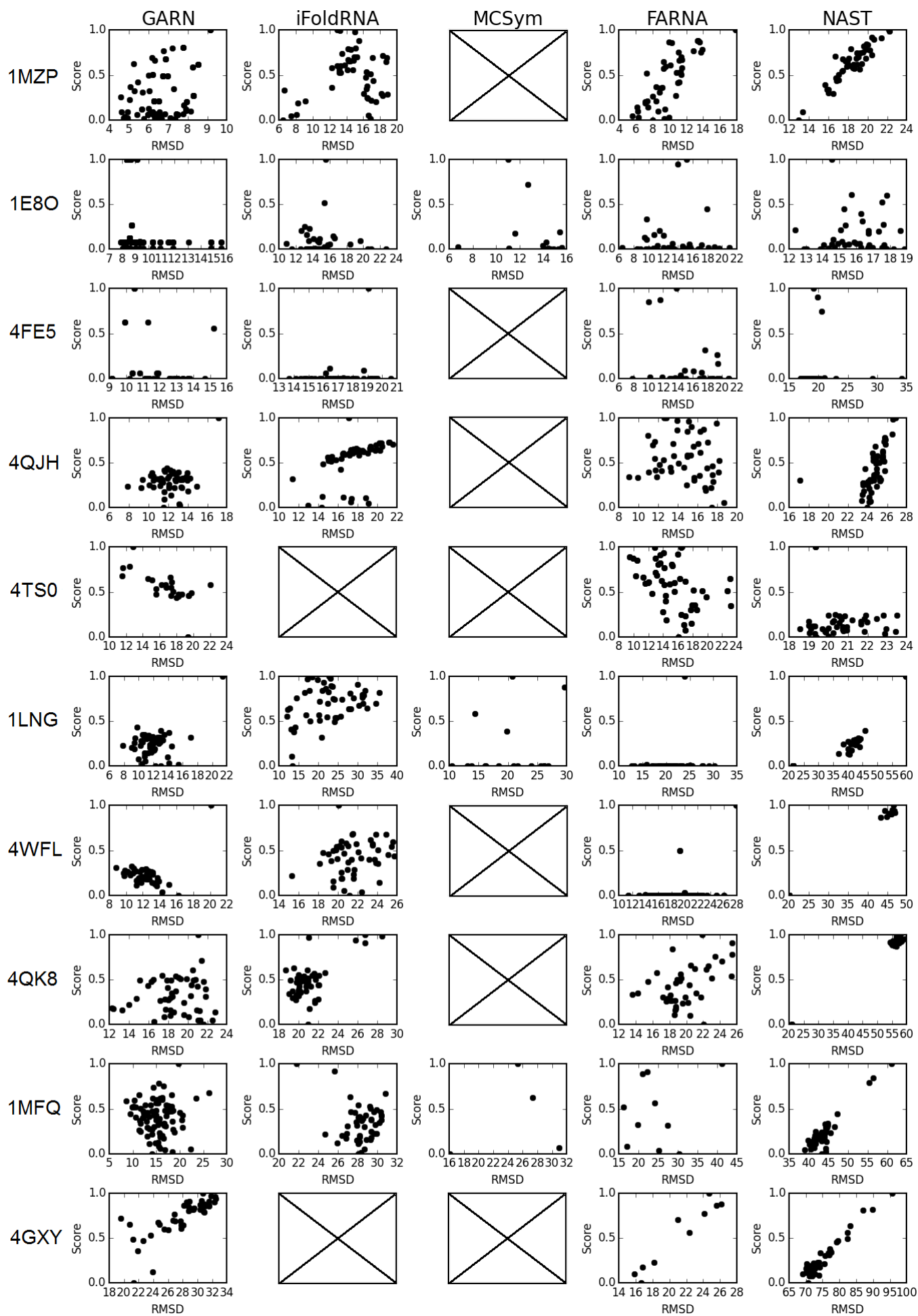
Figure S12: Energy vs. RMSD curves for the test set . Energy is calculated as the default GARN score multiplied by -1 and normalized.
