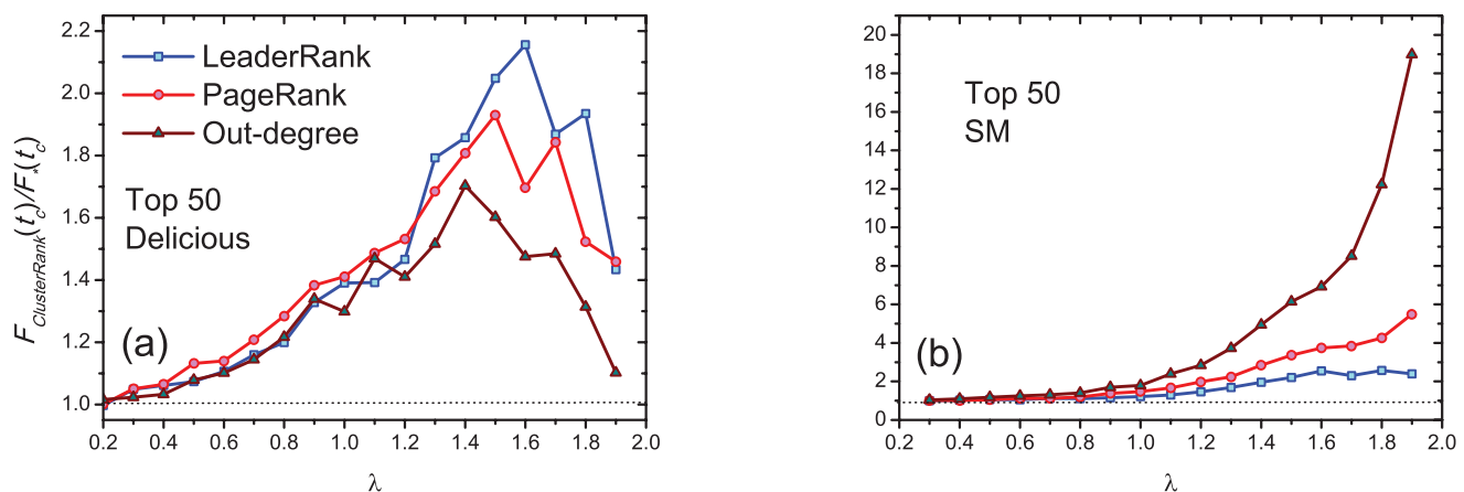
Figure 7. The ratio of the number of final recovered nodes by ClusterRank to those by out-degree centrality, PageRank and LeaderRank. The non-overlapped nodes in the top-50 lists are initially infected. We set \beta = 1/\langle k^{out} \rangle . Each data point is obtained by averaging over 100 independent runs.
