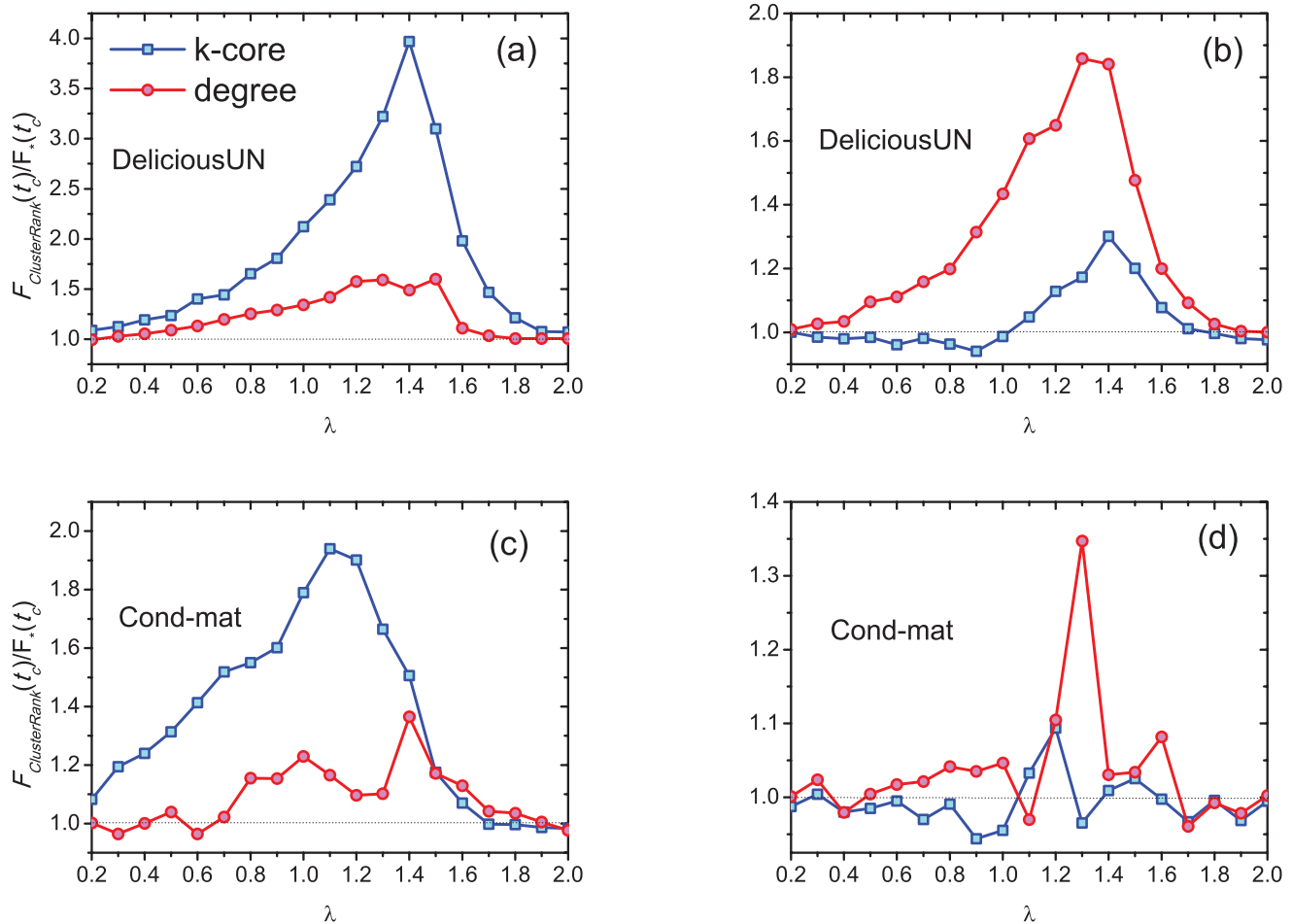
Figure 8. The dependence of F_{ClusterRank}(t_c)/F_*(t_c) on parameter \lambda in undirected Delicous and Cond-mat networks. We set \beta = 1/\langle k \rangle . In (a) and (c), the initial infected nodes are those non-overlapped nodes in the top-50 places regardless of whether they are connected or not. In (b) and (d), the initial infected nodes are the non-overlapped nodes in top-50 places under constraint that any two of them are not connected. Each data point is obtained by averaging over 100 independent runs. doi:10.1371/journal.pone.0077455.g008
