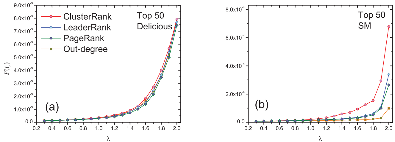
Figure 6. The dependence of F(t_c) on parameter \lambda . The initially infected nodes are the top-50 nodes obtained by out-degree centrality (squares), PageRank (diamonds), LeaderRank (triangles) and ClusterRank (circles). We set \beta = 1/\langle k^{out} \rangle . Each data point is obtained by averaging over 100 independent runs.
