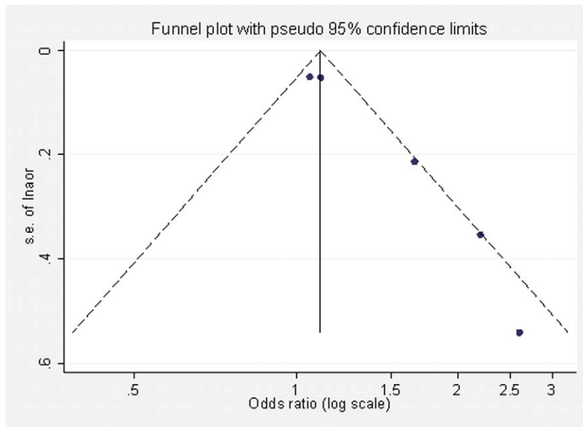
Figure 2. Funnel plot of the effect estimates (ln OR) by their SEs (s.e. of ln OR). The vertical line indicates the summary effect estimate (1.11) from the fixed-effects model according to the SE, and the dashed lines show pseudo 95% confidence limits for the summary effect estimate. doi:10.1371/journal.pone.0033949.g002
