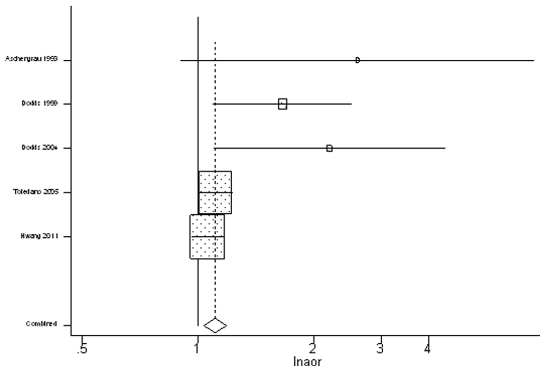
Figure 1. Tree Plots of Study-specific and Summary Effect Estimates for all available studies.
