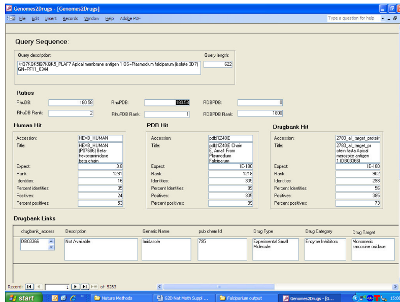
Supplementary Figure S1: Screen shots of the input and output of the online Genomes2Drugs tool.
