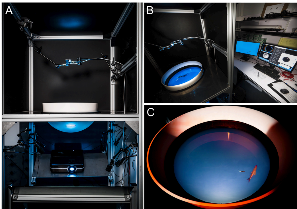
Fig 1. Analysis and modeling of interactions between schooling fish in a closed-loop virtual reality setup. (A) Closed-loop virtual reality setup used to measure and analyze in real time the interactions between fish within a school and their effects on individual behavior. (B) The virtual reality setup makes it possible to track in real time the 3D movements of a fish moving freely in a hemispheric tank. (C) These data then feed a mathematical model controlling the behavior and movement of one or several realistic virtual fish of the same species, the 3D anamorphic image of which being projected onto the hemispherical screen constituting the tank wall.
