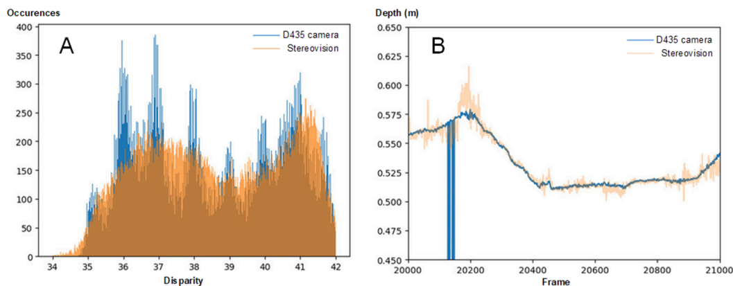
Fig 3. Disparities between the depth map and the stereo vision tracking modes. (A) Disparities computed with D435 camera (blue) and standard stereo vision (orange) for 10 min of tracking data. (B) Raw depth for a 1000-frame sample in the same experiment.
