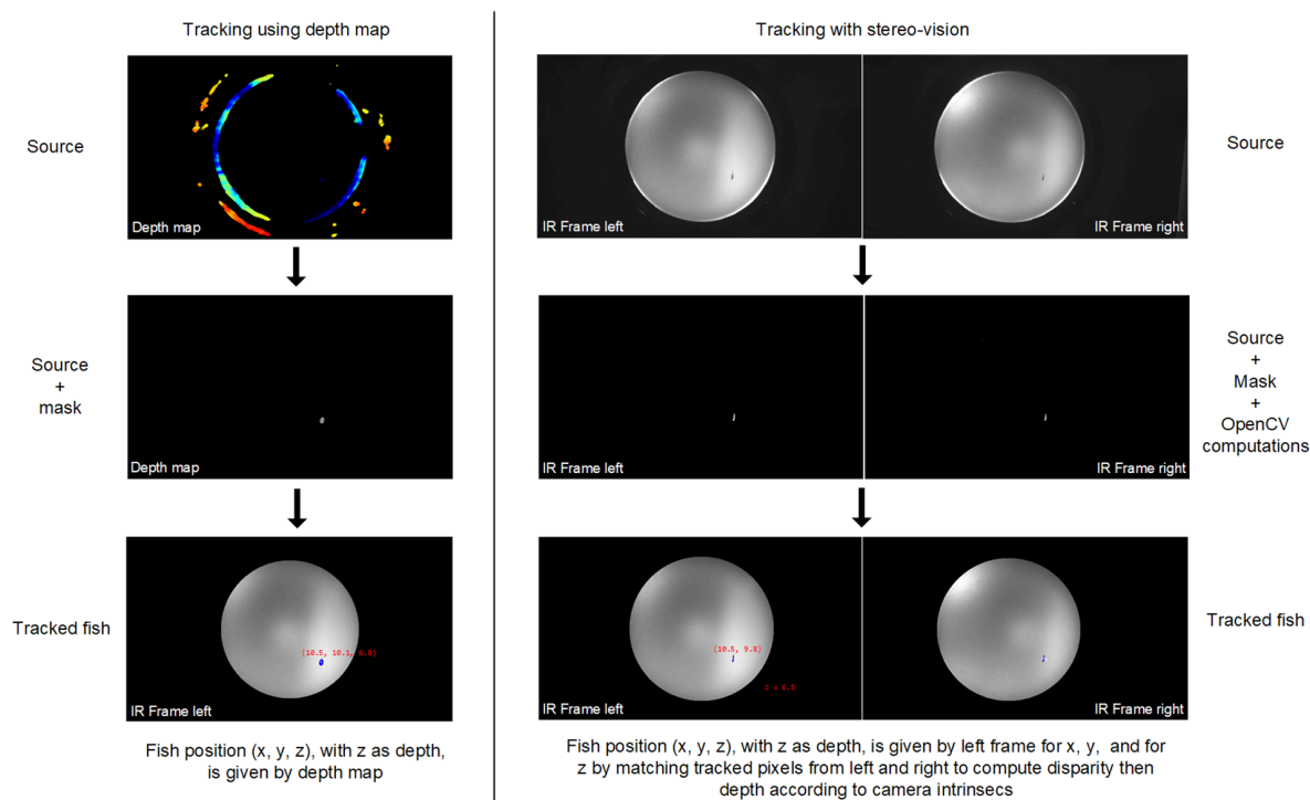
Fig 2. Operating modes of the 3D tracking. Detail of the tracking process for the same frame set using D435 camera computed depth map (left) and classical stereo-vision computation from left and right infrared frames (right).
