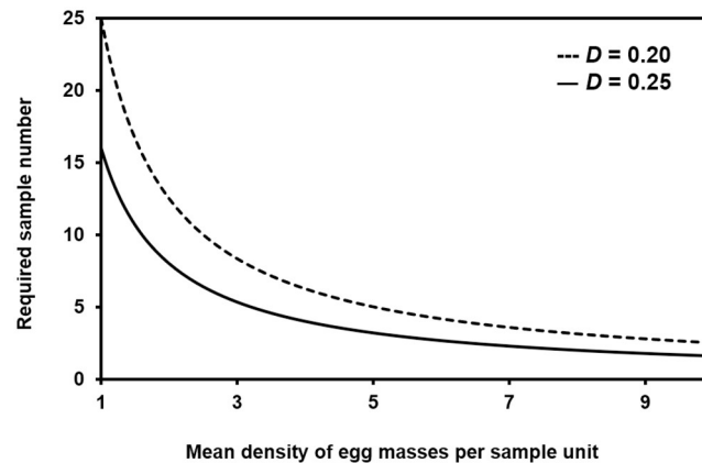
Fig 1. Required sample numbers according to mean densities of R. shantungensis egg masses in fixed precision level ( D ) of 0.20 and 0.25.
