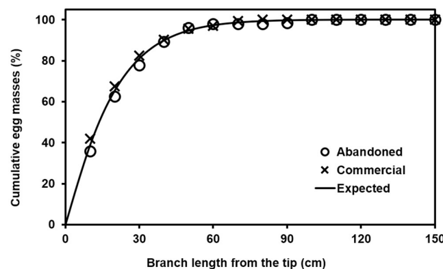
Fig 2. Cumulative egg mass proportion (%) of R. shantungensis according to distances from the tip within a branch.
