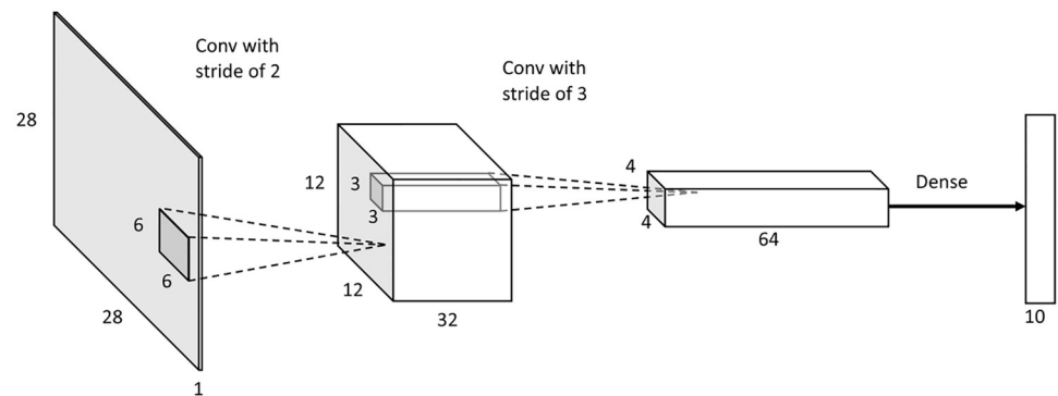
Fig 2. Architecture of our best SNN.
