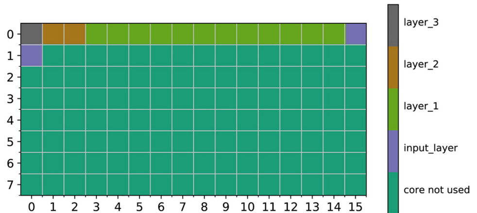
Fig 3. SNN layer distribution on Loihi chip.
