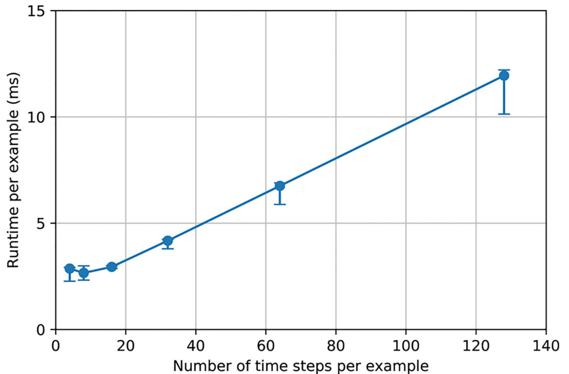
Fig 5. Tradeoff between runtime and number of time steps.
