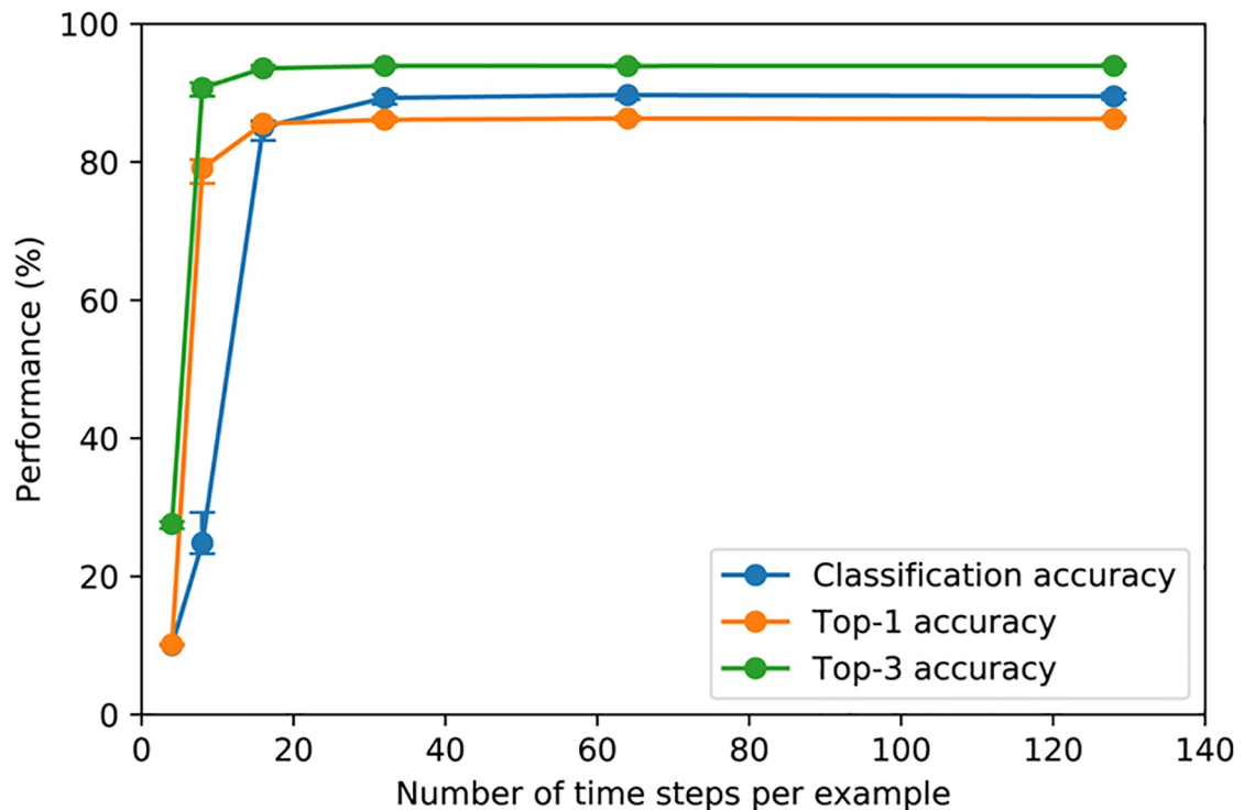
Fig 4. Tradeoff between performance metrics and number of time steps.
