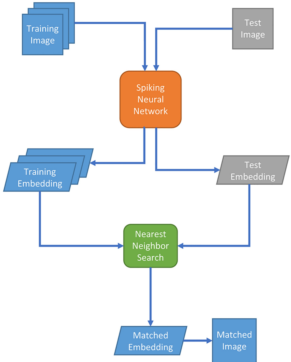
Fig 1. Pipeline of image retrieval by spiking neural network.
