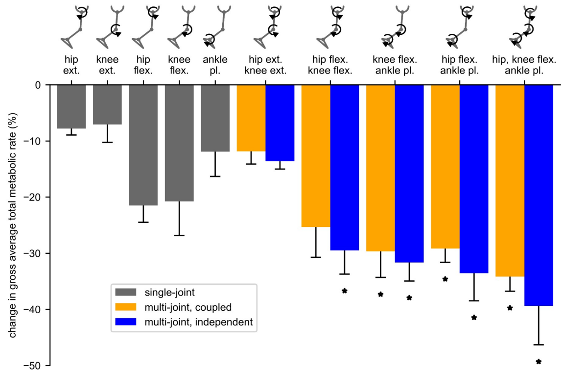
Fig 1. Reduction in metabolic rate for single and multi-joint assistance devices. The percent change in gross total metabolic rate, averaged over the gait cycle, for the single joint (gray), multi-joint coupled (orange), and multi-joint independent (blue) assistance devices. Negative values indicate decreases in metabolic cost. Each bar value and corresponding error bar provides the mean reduction and standard deviation across subjects. Asterisks indicate devices that produced significantly larger metabolic reductions compared to single-joint devices.
