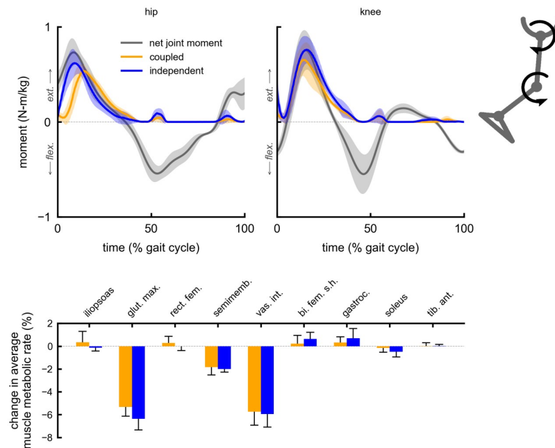
Fig 2. Summary of multi-joint hip-extension knee-extension assistance. Top: the device torques for multi-joint hip-extension knee-extension assistance with coupled (orange) and independent (blue) control compared to net joint moments (gray). Bottom: changes in average muscle metabolic rates as a percent of unassisted gross average total metabolic rate for the multi-joint assistive devices. Negative values indicate decreases in metabolic cost. Solid bars and error bars indicate the mean and standard deviation across subjects, respectively. Summing the individual muscle percent changes yields the total percent changes for the hip-extension knee-extension multi-joint devices reported in Fig 1.
