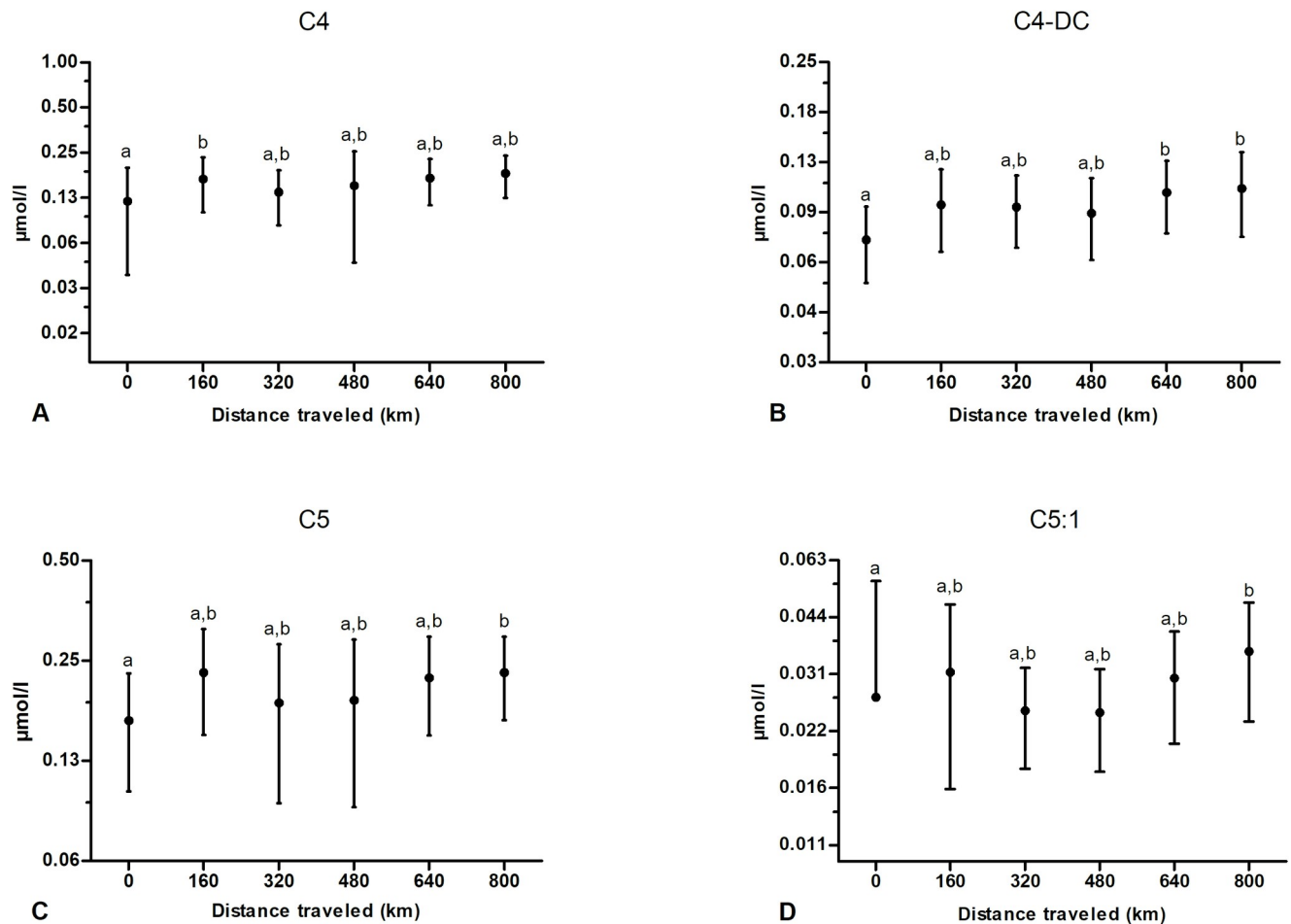
Fig 2. Effect of multiday exercise on some plasma short-chain acylcarnitines (SCACs). Samples were obtained from 9 dogs at 0, 160, 320, 480, 640 and 800 km. Data are displayed as raw data (mean \pm SD) on a logarithmic axis. Columns with different superscripts (a, b) are significantly different between them ( P < 0.05 ) and not significantly different from columns with the same superscript. Missing low error bars correspond to negative values that cannot be displayed on a logarithmic axis.
