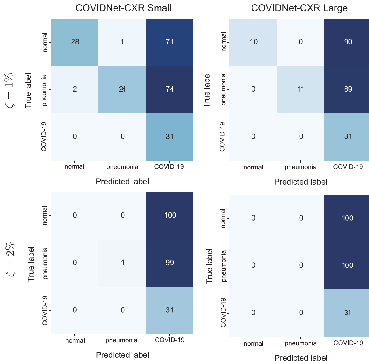
Fig 1. Confusion matrices for the COVID-Net models attacked using the non-targeted UAPs on the test images. p = \infty . Left and right panels represent the COVIDNet-CXR Small and COVIDNet-CXR Large models, respectively. The top and bottom panels indicate \zeta = 1\% and \zeta = 2\% , respectively.
