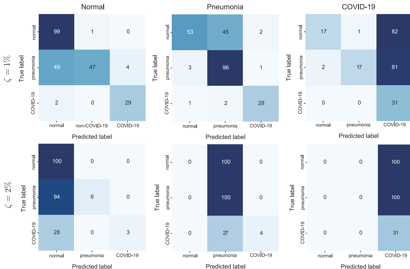
Fig 3. Confusion matrices for the COVIDNet-CXR Small model attacked with the targeted UAPs with p = \infty on the test images. The left, middle, and right panels represent the targeted classes: normal , pneumonia , and COVID-19 , respectively. The top and bottom panels indicate \zeta = 1\% and \zeta = 2\% , respectively.
