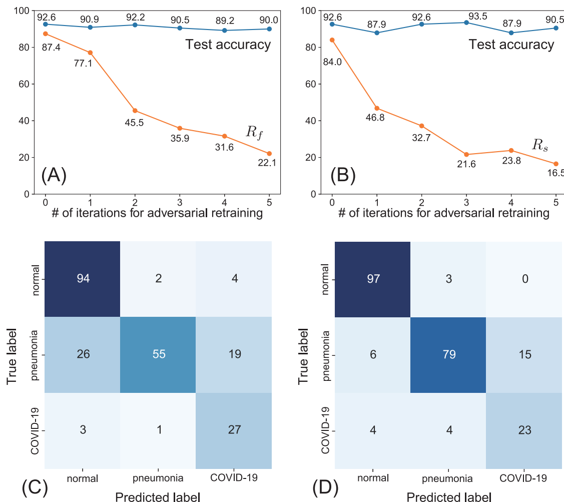
Fig 5. Effect of adversarial retraining on the robustness to UAPs with p = \infty against the COVIDNet-CXR Small model. Scatter plots of (A) the fooling rate, R_f (%), for non-targeted UAPs with \zeta = 2\% versus the number, N_i , of iterations for adversarial retraining and (B) the targeted attack success rate, R_s (%), of targeted UAPs with \zeta = 1\% to COVID-19 versus N_i . Here, R_f and R_s are for the test images. The accuracies (%) on the set of clean test images are also shown. The confusion matrices for the fine-tuned models were obtained after five iterations of adversarial retraining using the (C) non-targeted UAPs and (D) targeted UAPs. Note that these confusion matrices belong to the fine-tuned models attacked using non-targeted and targeted UAPs, respectively.
