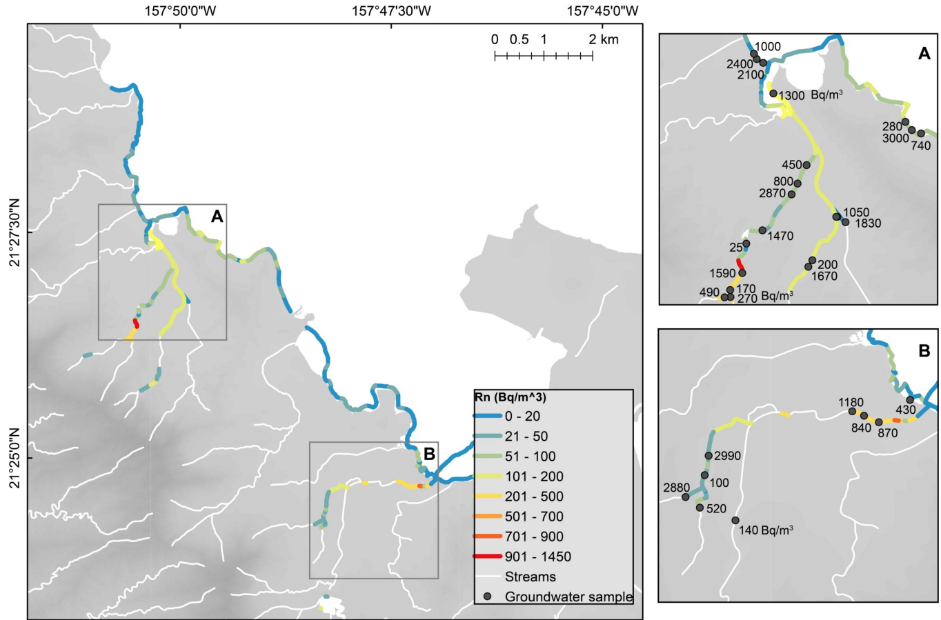
Fig 4. Non-modeled coastal and stream surface radon ( \text{Bq/m}^3 ) concentrations for Kāne'ohe Bay and studied streams (July sampling period). Stream surface radon concentrations (lines) and discrete (dots) groundwater radon concentrations are shown for (A) Kahalu'u and 'āhuimanu and (B) Kāne'ohe areas.
