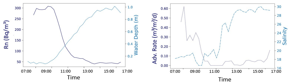
Fig 5. Radon time series. Radon (dark blue, in Bq/m 3 ) and water depth (light blue, in m), and three-point running average advection rates (m 3 /m 2 /d) and salinity time series from low to high tide. Results from (A) May 26, 2017 (perigean spring tide, tidal range = 0.09 to 0.99 m) from Kahalu'u estuary, (B) June 14, 2017 (spring tide, tidal range = 0.03 to 0.69 m) from Kahalu'u Beach Park, (C) June 23, 2017 (perigean spring tide, tidal range = 0.02 to 1.01 m) from the same location at Kahalu'u Beach Park.
