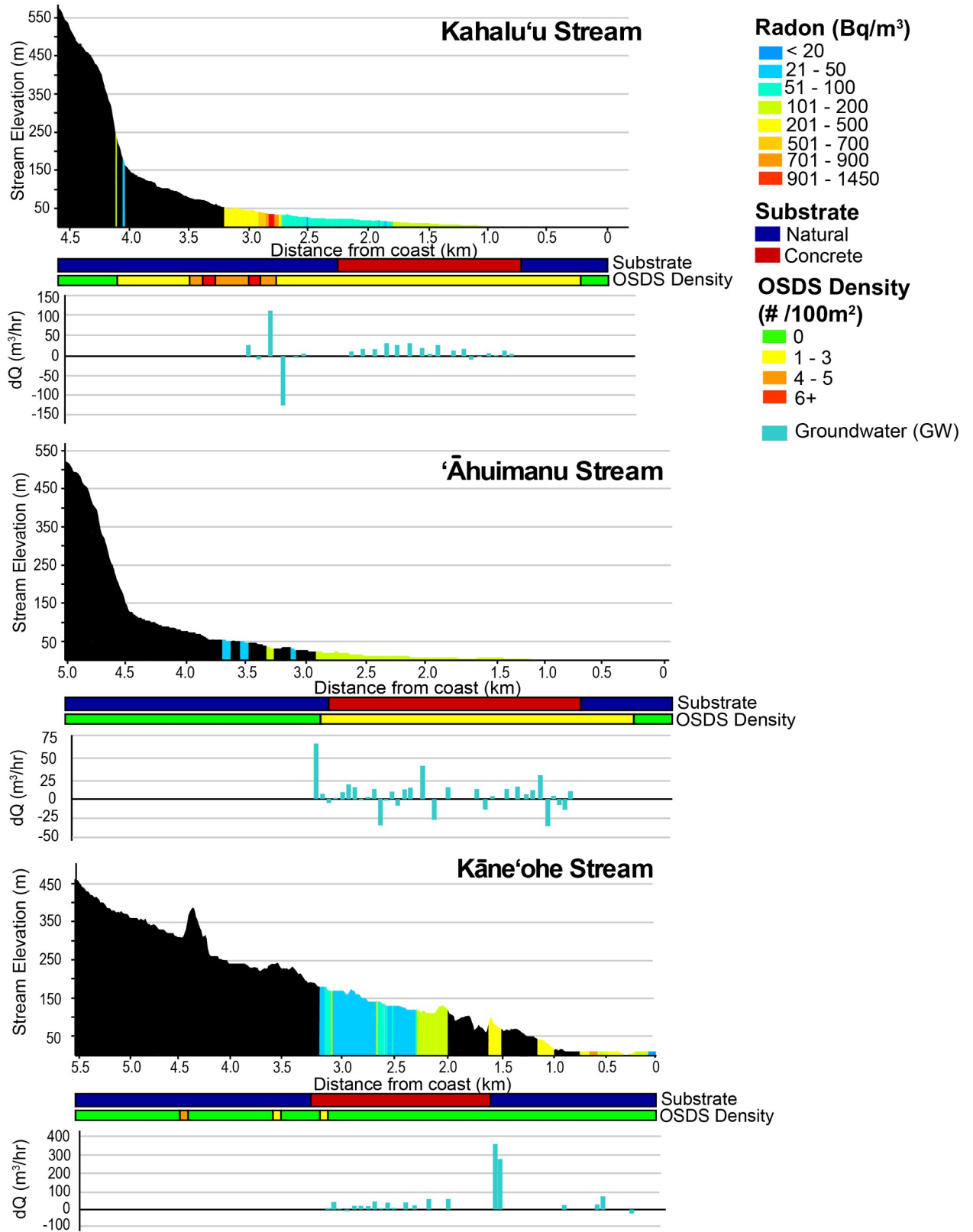
Fig 6. Groundwater fluxes in Kahalu'u, 'ahuimanu, and Kane'ohē Streams (using non-modeled results) for the July sampling period. Stream elevation [59] is shown in m with surface water radon concentrations overlain in Bq/m 3 . Stream substrate (natural–blue, concrete–red) and the
