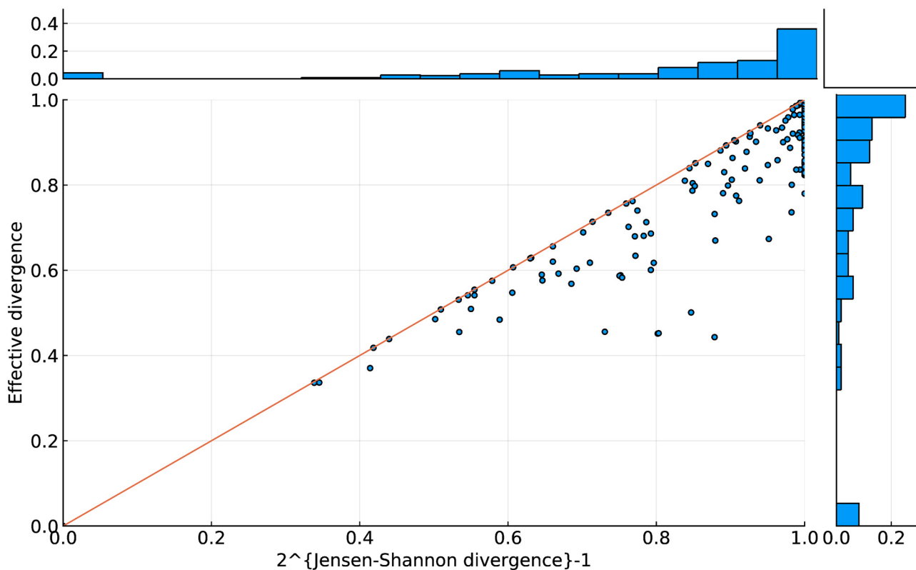
Fig 6. A comparison of the two entropy-based distance metrics showing that the intuitive divergence \bar{D}_{intuitive} lies below the Jensen-Shannon measure \bar{D}_{JS} (each point corresponds to one pair of movies).
