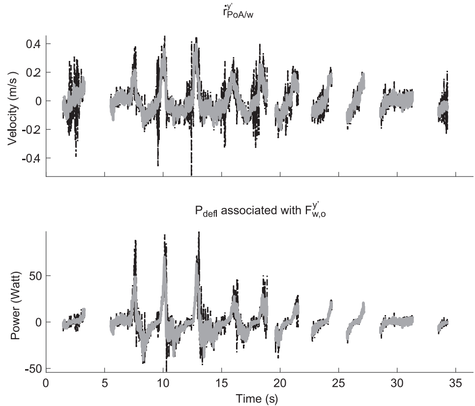
Fig 5. Typical examples of (a) the velocity in y' -direction of the location of the blade where the point of application is located ( \vec{r}'_{PoA/w} ), and (b) the component of P_{defl} associated with the perpendicular force. The bold grey lines represent the reference values obtained using Optotrak and the force transducer, while the black dashed lines are the values obtained using the presented method. Note that the missing data is data in which the parallel force is lower than -30 N and higher than 20 N.
