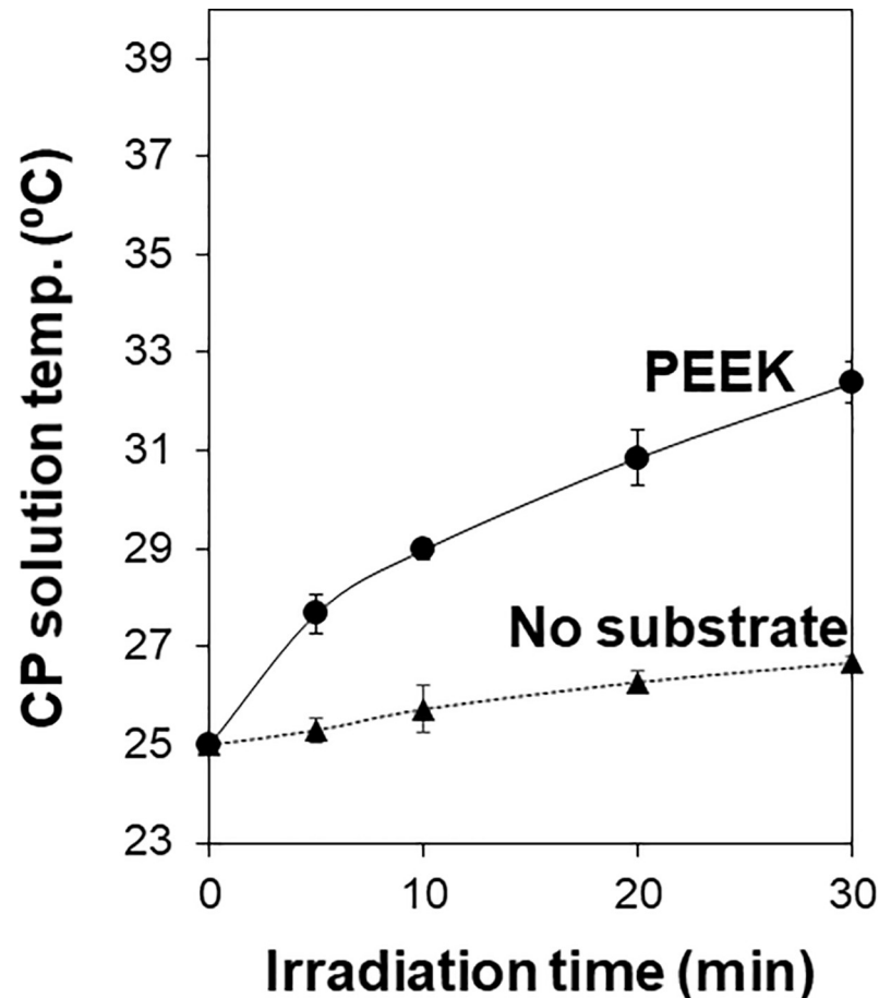
Fig 6. Temperature variations of the CP solution with and without the PEEK substrate during laser irradiation at 2 \text{ W/cm}^2 without a temperature-controlled water bath. Data are expressed as the average \pm standard deviation ( n = 4 ).
