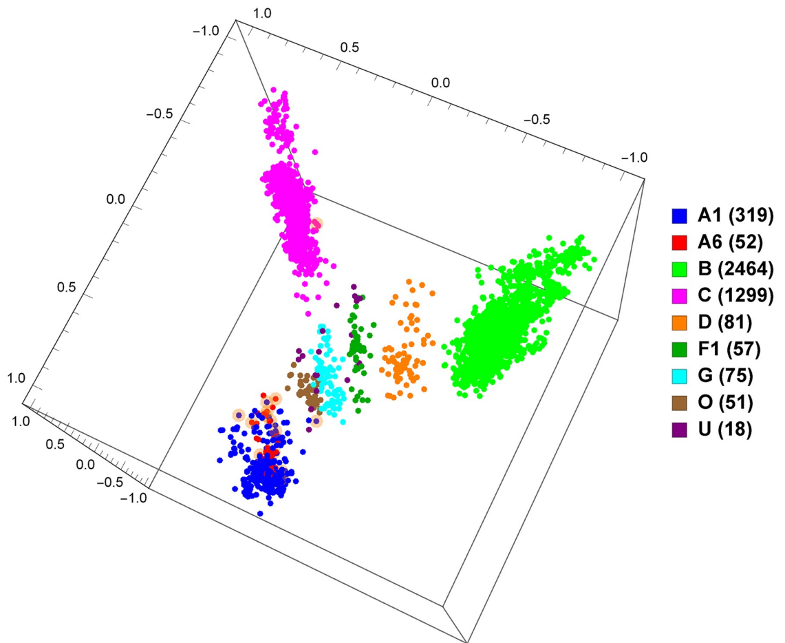
Fig 2. MoDMap of 4373 full-length HIV-1 genomes of 9 different pure subtypes or groups, at k = 6 .
