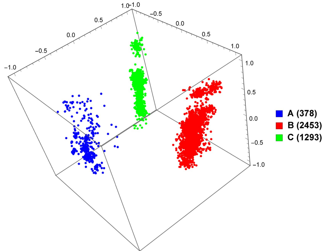
Fig 3. MoDMap of 4124 full-length HIV-1 genomes of subtypes A, B, and C, at k = 6 .
