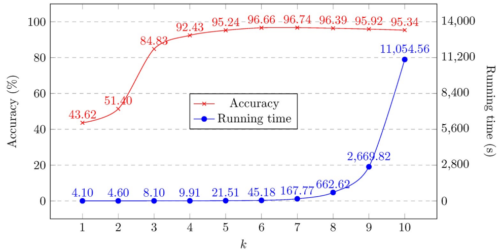
Fig 1. Highest accuracy score and running time averaged across all fifteen classifier algorithms, at different values of k , for the full set of 6625 whole HIV-1 genomes from the LANL database.
