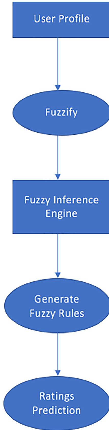
Fig 3. Fuzzy algorithm.
