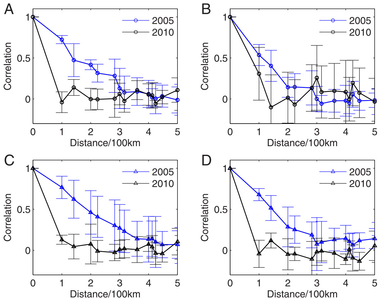
Fig 9. Correlation distances to the ROI at (58° W, 8.5° S) in the extreme drought network (A, B), and respectively, to the ROI at (65° W, 5.5° S) in the network of normal drought conditions (C, D). (A, C) summer, and (B, D) winter. Error-bars correspond to the standard deviations.
