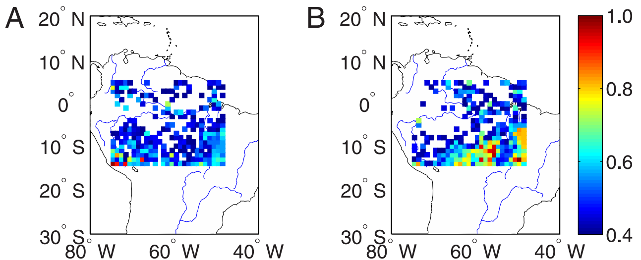
Fig 3. Distribution of 50% large values of drought strength across the Amazon region in the year (A) 2005, and (B) 2010.
