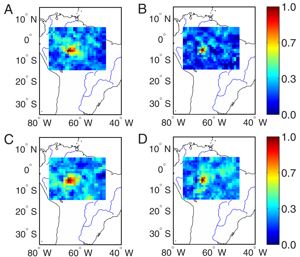
Fig 8. Map of correlation coefficients to the ROI at (65° W, 5.5° S) as indicated by x, where large network degrees are observed in the network of normal drought conditions. (A) austral summer 2005, (B) winter 2005, (C) summer 2010, and (D) winter 2010.
