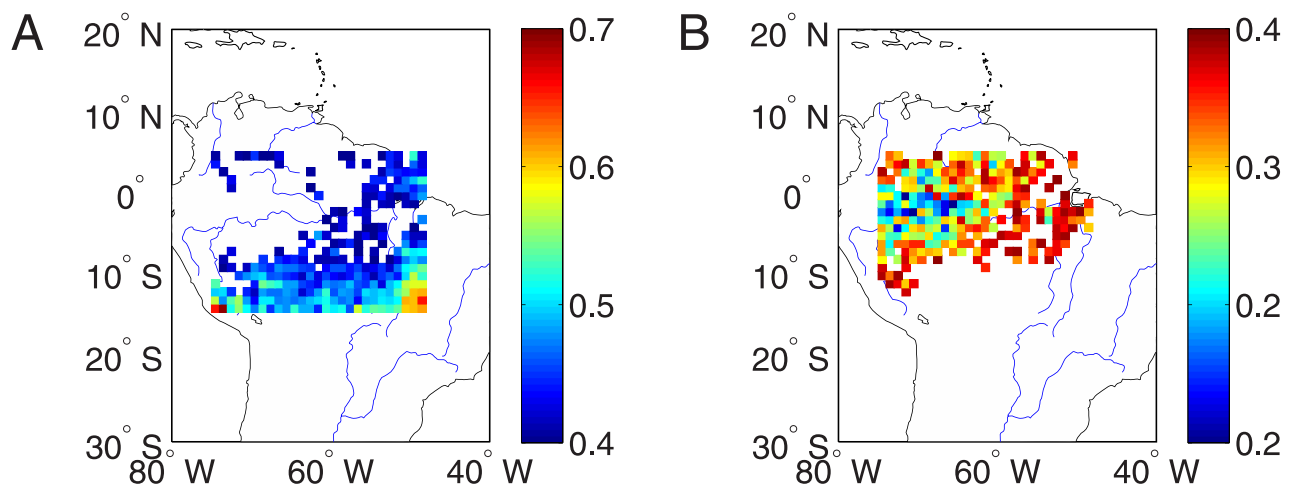
Fig 5. Maps of averaged NDS values. Locations of (A) 50% upper quantile and (B) 50% lower quantile of NDS values.
