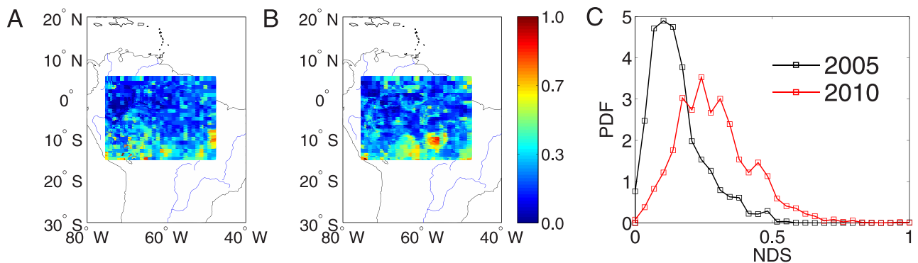
Fig 1. Normalized drought strength over Amazon region. (A) 2005, (B) 2010, and (C) probability distribution functions of normalized drought length.
