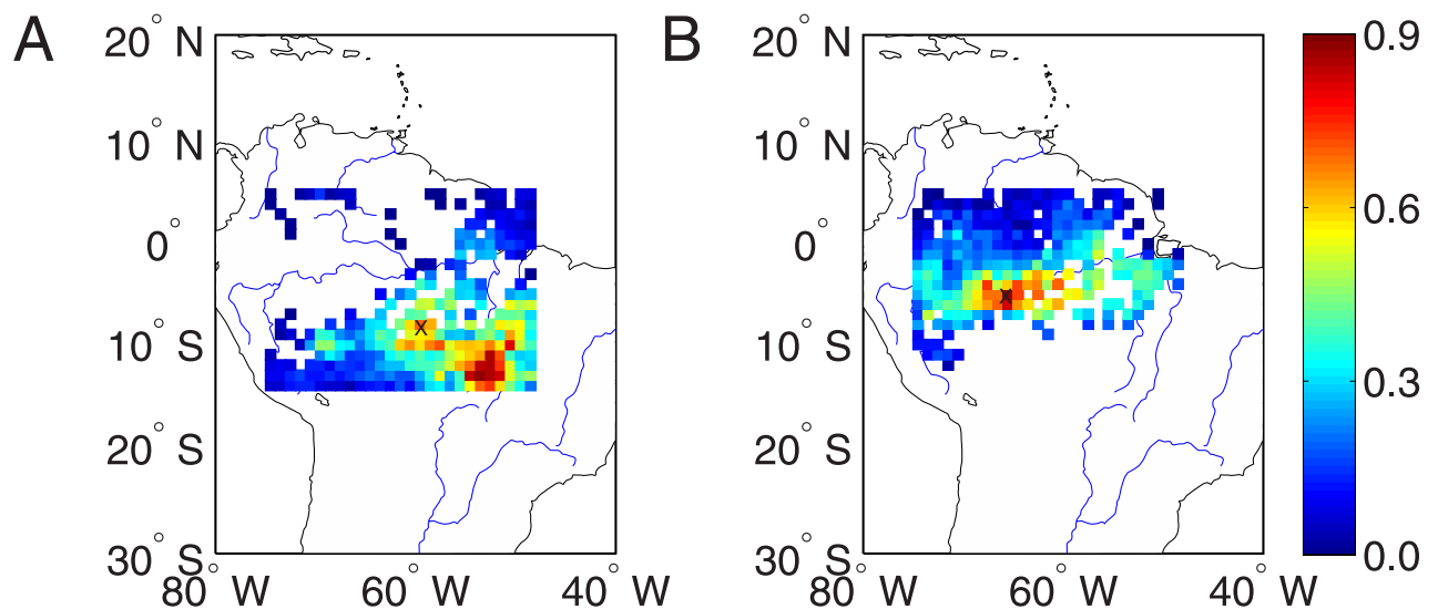
Fig 6. Map of the averaged network degrees (normalized to unit interval) for locations that are characterized by 50% upper quantile of NDS values (A), and (B) 50% lower quantile of NDS values. The ROIs are denoted by x.
