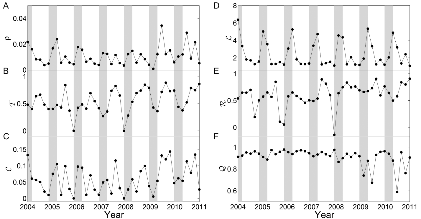
Fig 2. Network measures and gray areas highlight the austral summer periods. (A) link density \rho , (B) transitivity T , (C) clustering coefficient C , (D) average path length L , (E) assortativity R and (F) modularity Q . Gray time windows highlight the summer seasons.
