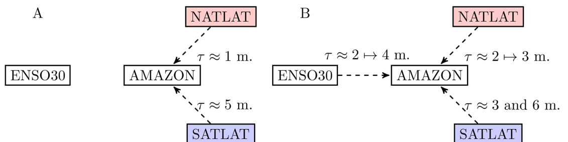
Fig 10. Delays of the ocean effects on the precipitations in the Amazon. (A) 2005, no significant delay effects have been identified from the ENSO region, and (B) 2010.
