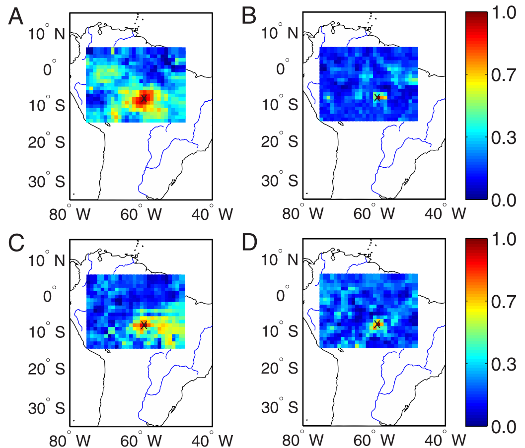
Fig 7. Map of correlation coefficients to the ROI at (58° W, 8.5° S) as indicated by x, where large network degrees are observed in the extreme drought networks. (A) austral summer 2005, (B) winter 2005, (C) summer 2010, and (D) winter 2010.
