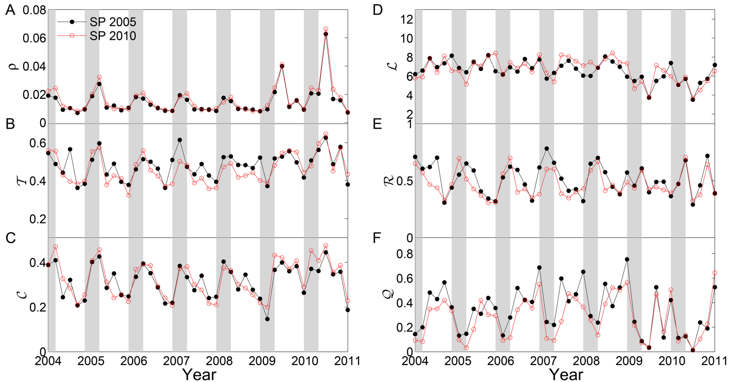
Fig 4. Network measures of extreme drought networks. Gray areas highlight the austral summer periods (• spatial points of 2005, and ° spatial points of 2010). (A) link density \rho , (B) transitivity \mathcal{T} , (C) clustering coefficient \mathcal{C} , (D) average path length \mathcal{L} , (E) assortativity \mathcal{R} and (F) modularity \mathcal{Q} . Gray time windows highlight the summer seasons.
