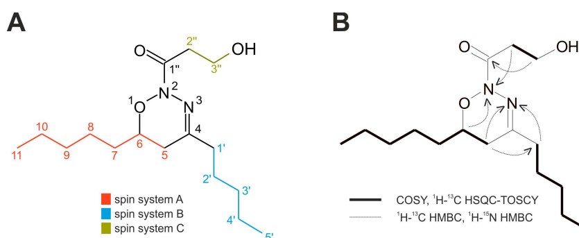
Fig 1. Chemical structure of nocuolin A. Panel (A) demonstrates nocuolin A molecule with highlighted spin systems A, B, and C as obtained by NMR—COSY and ^1\text{H} - ^{13}\text{C} HSQC-TOCSY. Panel (B) displays the crucial NMR correlations. See also S1–S12 Figs. High resolution mass spectrometry (HRMS) measurement of NoA provided ions corresponding to a protonated molecule [\text{M}+\text{H}]^+ , sodium adduct [\text{M}+\text{Na}]^+ , potassium adduct [\text{M}+\text{K}]^+ , and sodium adduct of a dimer [2\text{M}+\text{Na}]^+ (S2 Fig), which allowed us to determine the exact mass of the protonated molecule (299.2233) and to calculate the neutral formula to \text{C}_{16}\text{H}_{30}\text{N}_2\text{O}_3 with high accuracy ( \Delta 1.2 ppm in FTMS). In parallel we have found production of this compound in extracts of two other cyanobacterial strains, Anabaena sp. PCC 7108 (axenic strain) and Nodularia sp. HBU26, via HPLC-HRMS/MS measurements (S1B and S1C Fig). The analysis revealed the occurrence of a molecular ion perfectly matching that of NoA in molecular mass, fragmentation pattern and retention behaviour in extracts of both strains (S1 Fig). However, due to the extremely low level of NoA production in PCC 7108 and HBU26 we have performed the structure elucidation on the compound purified from strain Nostoc sp. CCAP 1453/38.
