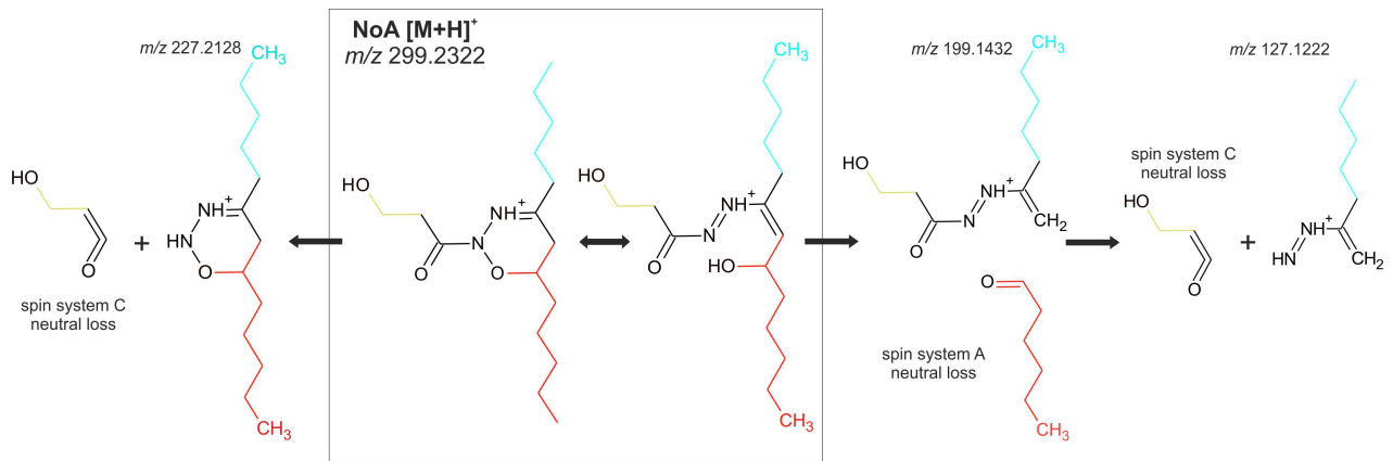
Fig 2. MS fragments of nocuolin A demonstrating the connection of the A/B and C spin systems obtained by NMR. We suppose the formation of secondary linear resonance structure with interrupted N-O bond of the oxadiazine ring and formation of additional N-N double bond during the ionization process. For the full MS spectra see S2 Fig and for detail fragmentation see S10 Fig .
