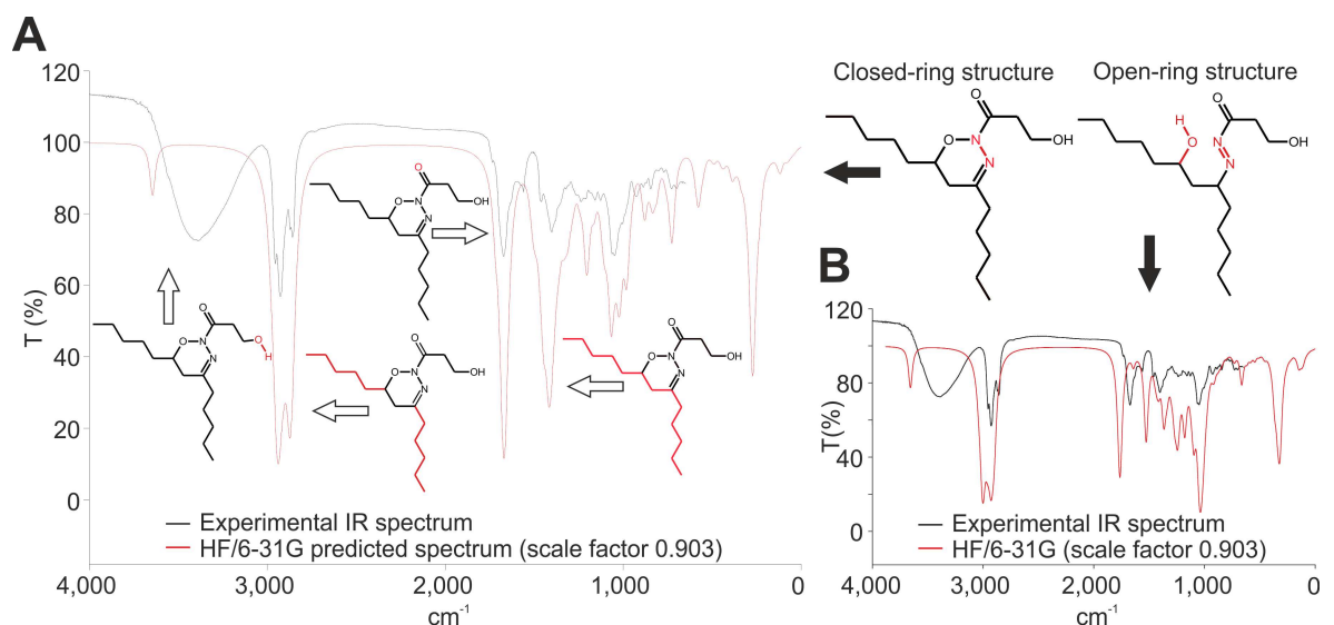
Fig 3. Predicted and experimental FTIR spectra of cyclic nocuolin A form (A) and hypothetical linearized structure (B). In the case of cyclic NoA form the theoretically predicted ab initio spectrum (red line) show exceptionally good overlap with the experimental (black line). Substantially different was the predicted spectrum seen for hypothetical linear NoA form. The main vibration bands and corresponding structures are highlighted. For details see S11 and S12 Figs .
