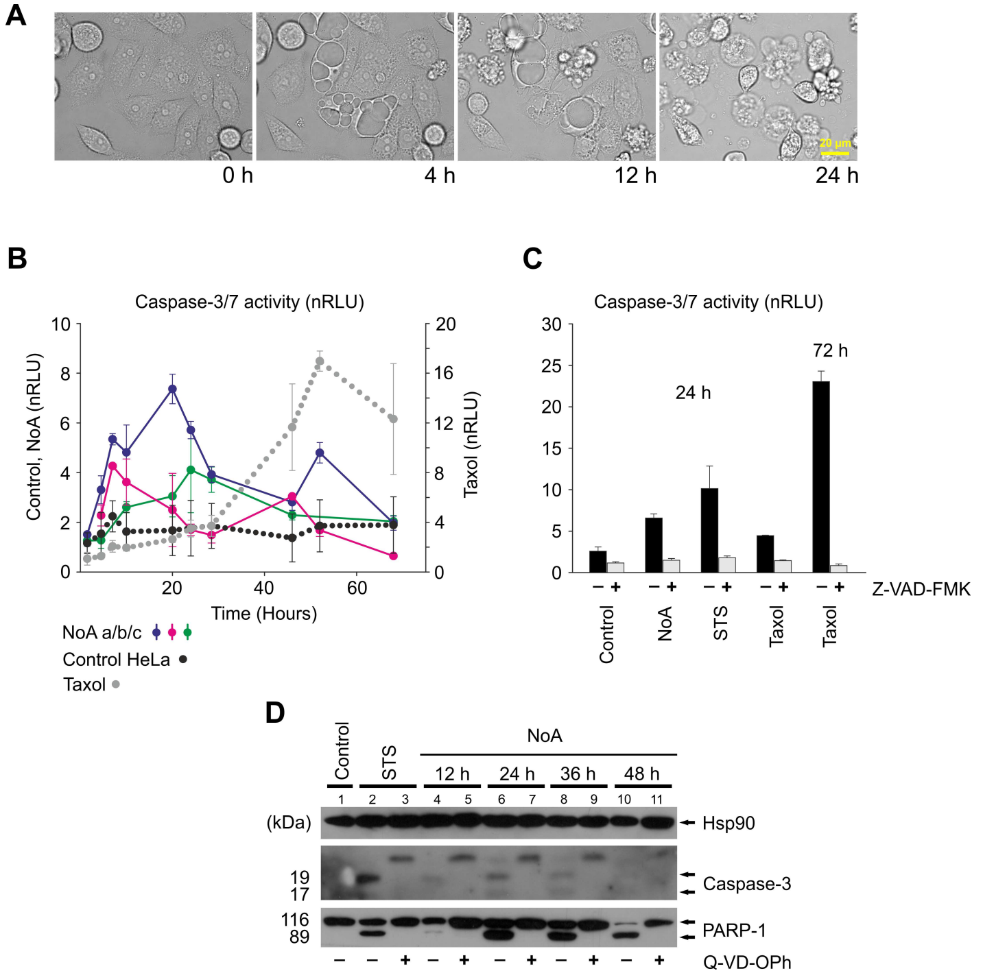
Fig 4. Nocuolin A triggers caspase-dependent apoptosis. (A) NoA-induced cell death morphologically resembles apoptosis (blebbing) as illustrated by the time-lapse microscopy images obtained with HeLa cells exposed to 6.7 \mu M NoA over 24 hours. (B, C, D) The cell death is caspase-dependent. (B) The protease activity of caspase-3/7 for the DEVD sequence was measured as a luminescence signal at various time points. The relative luminescence units were normalised per cell (nRLU). NoA (a/b/c) at 6.7 \mu M stands for three independent experiments. (C) The enhanced activity of caspase-3/7 (nRLU) was reduced when the cells treated with NoA and positive controls, were pre-treated with caspase inhibitor Z-VAD-FMK (10 \mu M). (D) NoA treatment (6.7 \mu M) resulted in weak enhancement of activated caspase-3 fragments (19/17 kDa) and a consistent increase in PARP-1 cleavage. These apoptosis markers were completely absent when the caspase inhibitor Q-VD-Oph (10 \mu M) was added prior to NoA (lines 5,7,9,11). As a positive control, taxol (B) and staurosporine (STS) (C, D) were used both at concentration 1 \mu M and for indicated time.
