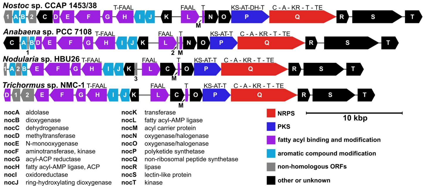
Fig 5. Structure of the noc gene cluster in four cyanobacterial strains. Gene arrangement, functional annotation of nocA–T genes, and domain structure of the PKS/NRPS genes. A—adenylation domain; AT—acyltransferase; C—condensation domain; DH—dehydratase domain; FAAL—fatty acyl-AMP ligase; KR—ketoreductase; KS—ketosynthetase; NRPS—non-ribosomal peptide synthetase; PKS—polyketide synthetase; T—thiolation domain (acyl or peptidyl carrier protein); TE—thioesterase. See also S1 Table.
