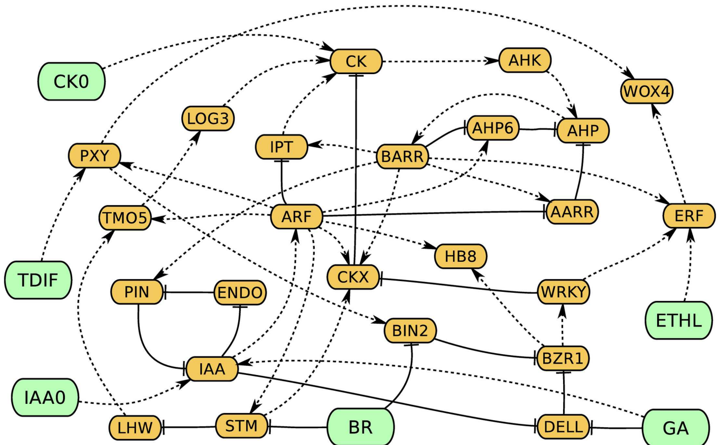
Fig 1. Cambium regulation gene network (CARENET). Control nodes are in green and internal nodes are in orange. Dashed and solid lines indicate activation and inhibition respectively. ATHB8 is labelled as HB8, ENDO means endocytosis.
