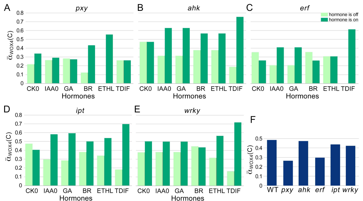
Fig 5. Effect of mutations on CARENET activity. A-E, Simulating effect of hormones on \bar{\alpha}_{WOX4}(C) in pxy , ahk , erf , ipt , and wrky mutant backgrounds. \bar{\alpha}_{WOX4}(C) was averaged for all the simulations with the corresponding control node on (dark green bar) or off (pale green bar). F, Proliferation in pxy , ahk , erf , ipt , and wrky mutant backgrounds.
