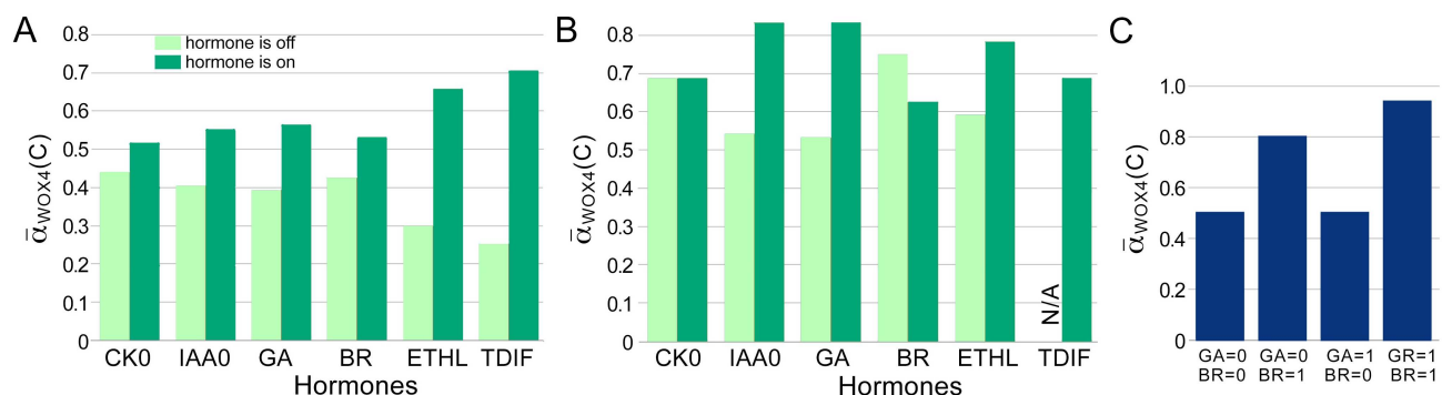
Fig 4. Effect of hormones on CARENET activity. A, \bar{\alpha}_{WOX4}(C) obtained in the simulations experiments where corresponding hormone (control node) is turned on (dark green bars) or off (pale green bars). B, \bar{\alpha}_{WOX4}(C) obtained in the simulations experiments where TDIF was always on (TDIF = 1) and corresponding hormone is turned on (dark green bars) or off (pale green bars). N/A, not applicable. C, Effect of gibberellins and brassinosteroids on \bar{\alpha}_{WOX4}(C) under conditions when the rest of the control nodes were on.
