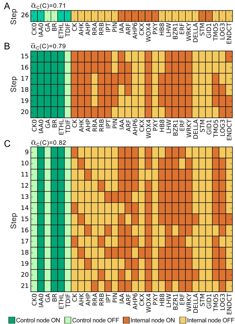
Fig 3. Representative examples of a stable state and limit cycles. A, Stable state achieved by step 26. B, C, Limit cycles established by step 15 or 9 respectively. Intracellular cytokinin (CK) synthesis oscillates even in the absence of external cytokinin CK0. ATHB8 is labelled as HB8.
