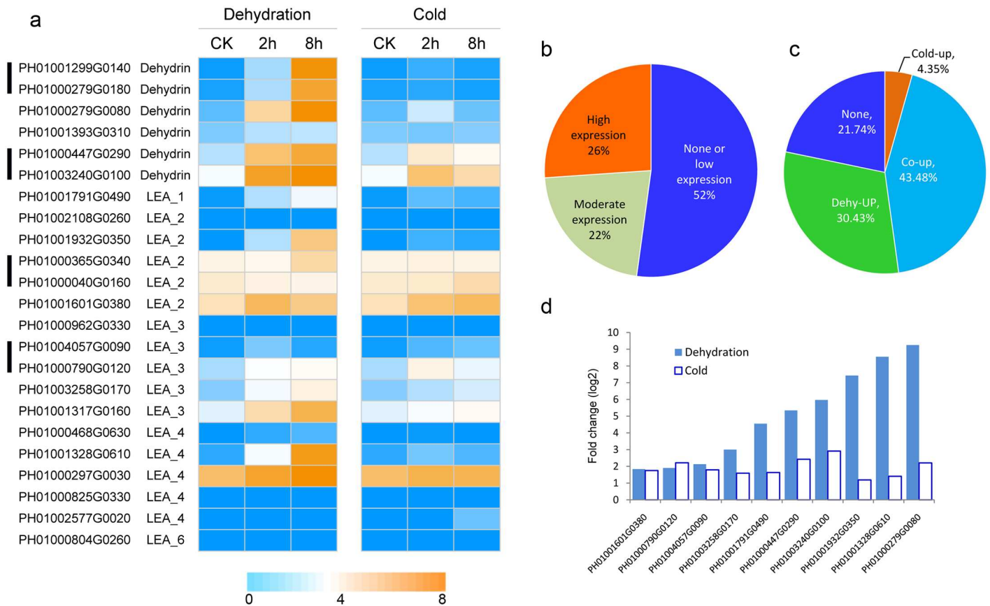
Fig 5. Expression profiling of PeLEA family under dehydration and cold stresses. a, Heatmap of expression values (showed by \log_2 RPKM values) in control, and in treated samples 2h and 8h after treatment; b, Percentage of genes in different expression levels under normal conditions; c, Percentage of genes exhibiting different responses to dehydration and cold; d, Comparison of fold changes of co-upregulated genes under dehydration and cold stresses. The expression data is obtained through two biological replicates. The relatedness of two replicates was present in S1 Fig. The black bars on the left indicate paralogous genes.
