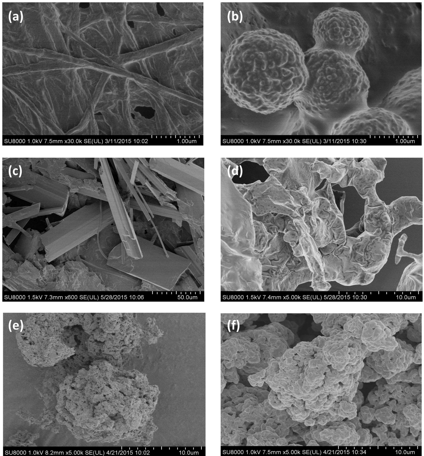
Fig 6. Polyaniline structures observed by SEM. Polymerization was carried out with 7D5L, 15 mM aniline and 5mM of different templates. Nanofibers obtained with SDBS (a). Granular spheres obtained with 5 mM AOT (b). Splinters obtained with 5 mM SDS (c). Amorphous agglomerates obtained with 5 mM SLES (d). Amorphous agglomerates obtained after washing (a) with ethanol (e). Micro-sized granular agglomerates of commercial PANI (f).
