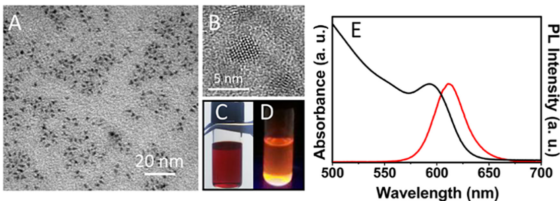
Fig 2. Preparation and characterization of ‘ as synthesized ’ CdSe@ZnS NCs. TEM (A) and HRTEM micrographs (B), absorption (E, black line) and PL (E, red line) spectra of organic capped CdSe@ZnS NCs dispersed in CHCl 3 . Picture of the sample under visible (C) and UV (D) light illumination.
