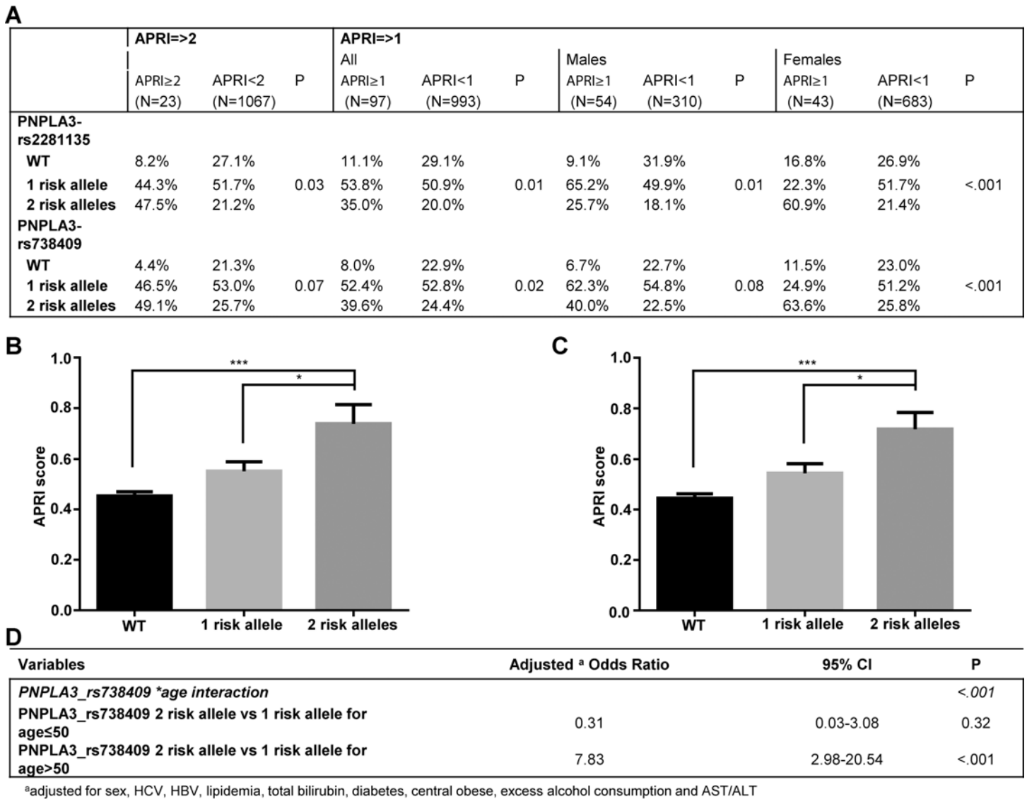
Fig 2. PNPLA3 SNPs and APRI scores. (A) PNPLA3 SNPs genotype distribution according to cirrhosis (APRI cutoff of 2) and cirrhosis/advanced fibrosis (APRI cutoff of 1) status. APRI scores in CCHC participants carrying PNPLA3 rs2281135 (B) and rs738409 (C) SNPs. (D) Association between PNPLA3 rs738409 and cirrhosis/advanced fibrosis (APRI cutoff of 1) based on multivariable logistic regression model. APRI = Aspartate transaminase to Platelet Ratio Index; SNP = single-nucleotide polymorphisms; PNPLA3 = patatin-like phospholipase domain-containing-3; CCHC = Cameron County Hispanic Cohort.
