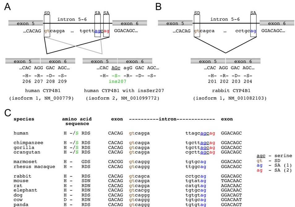
Fig 1. Alternative Splicing of CYP4B1 . (A) Human CYP4B1 . The human CYP4B1 intron 5–6 harbors two splice acceptors (SAs) in frame allowing the generation of two alternative CYP4B1 transcripts, with (isoform 2: NM_001099772) or without (isoform 1: NM_000779) insSer207. (B) Rabbit CYP4B1 . Intron 5–6 of rabbit CYP4B1 carries only a single SA and therefore generates a single transcript without insSer202 (isoform 1: NM_001082103). (C) Alignment of CYP4B1 sequences from other species. Alignment of the genomic DNA of CYP4B1 from other species shows that the insertion of the CAG triplet, which generates the additional splice acceptor site, exists only in humans and great apes, and not in rhesus, macaque, marmoset or other mammals.
