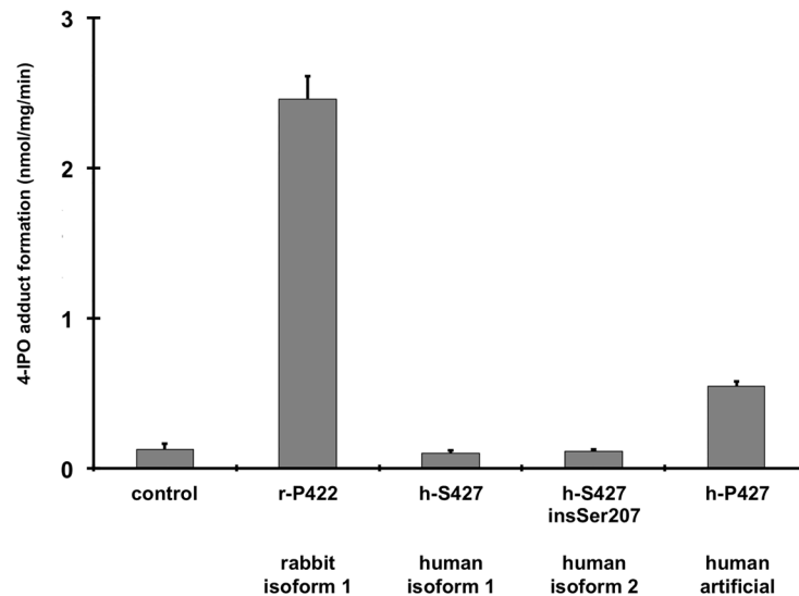
Fig 4. Bioactivation of 4-IPO to a stable NAC/NAL adduct. The NADPH-dependent formation of NAC/NAL adducts by membranes isolated from HepG2 cells stably transduced with the different CYP4B1 cDNAs r-P422: rabbit wild-type (isoform 1); h-S427: human wild-type (isoform 1); h-P427: human mutated p.S427P (artificial); h-S427 insSer207: human wild-type with insSer207 (isoform 2) after incubation in 50 nM 4-IPO for 20 minutes is shown. The adduct formation rate is shown as the mean \pm standard deviation (SD) of triplicate incubations.
