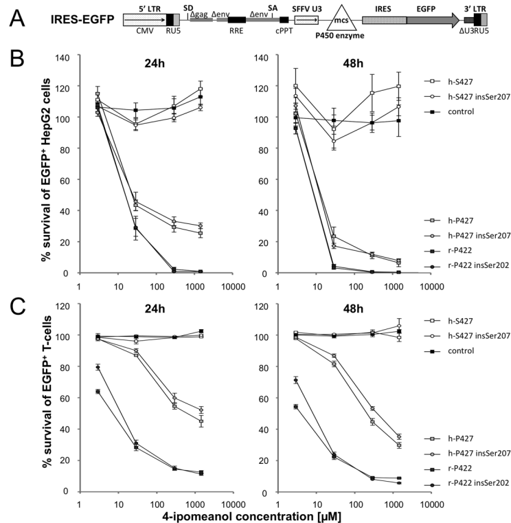
Fig 3. Functional analysis of CYP4B1. (A) Schematic outline of the lentiviral (LV) vectors used for expression of CYP4B1. For functional testing, the different CYP4B1 forms were cloned into a LV vector with an IRES-EGFP site. CMV: CMV promoter; SD: splice donor; LTR: long terminal repeat; SA: splice acceptor; RRE: Rev responsive element, cPPT: central polypurine binding tract; SFFV U3: U3 promoter of the spleen focus-forming virus; mcs: multicloning site; IRES: internal ribosomal entry site; EGFP: enhanced green fluorescent protein. (B) Toxicity of HepG2 cells after 4-IPO exposure. Survival of EGFP+ HepG2 cells (%) after 24 and 48 h of incubation with 0, 2.9, 29, 290 or 1450 μM 4-IPO as measured by flow cytometry. The cells stably expressed the different CYP4B1 enzymes: h-S427: human wild-type (isoform 1); h-S427 insSer207: human wild-type with insSer207 (isoform 2), h-P427: human mutated p.S427P (artificial); h-P427 insSer207: human mutated p.S427P with insSer207 (artificial); r-P422: rabbit wild-type (isoform 1); r-P422 insSer202: rabbit with insSer202 (artificial). For each construct, the mean ± standard error of the mean (SEM) values are shown from at least three independent experiments. The transduction efficiency of HepG2 cells (not shown) was ≥90%, as determined by EGFP expression in flow cytometry. (C) Toxicity of T cells after 4-IPO exposure. Survival of EGFP+ primary human T cells (%) expressing the different CYP4B1 proteins [listed for (B)] after 24 and 48 h of incubation with increasing doses of 4-IPO as assessed by flow cytometry. For each construct, the mean ± SEM values are shown from at least three experiments.
