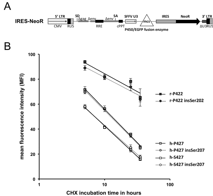
Fig 5. Protein stability of CYP4B1. (A) Schematic outline of the lentiviral vector used for expression of CYP4B1. CMV: CMV promoter; SD: splice donor; LTR: long terminal repeat; SA: splice acceptor; RRE: Rev responsive element, cPPT: central polypurine binding tract; SFFV U3: U3 promoter of the spleen focus-forming virus; mcs: multicloning site; IRES: internal ribosomal entry site; neoR: neomycin phosphotransferase (nptII) resistance cDNA; EGFP: enhanced green fluorescent protein. (B) Protein half-life analysis of CYP4B1 isoforms in HepG2 cells. Protein half-life analysis was performed by adding 50 µg/ml cycloheximide (CHX) to the transduced and G418-selected HepG2 cells. The mean fluorescence intensity (MFI) of CYP4B1/EGFP fusion proteins was assessed at various time points by flow cytometry. For each construct, the mean ± SEM values are shown from at least three experiments.
