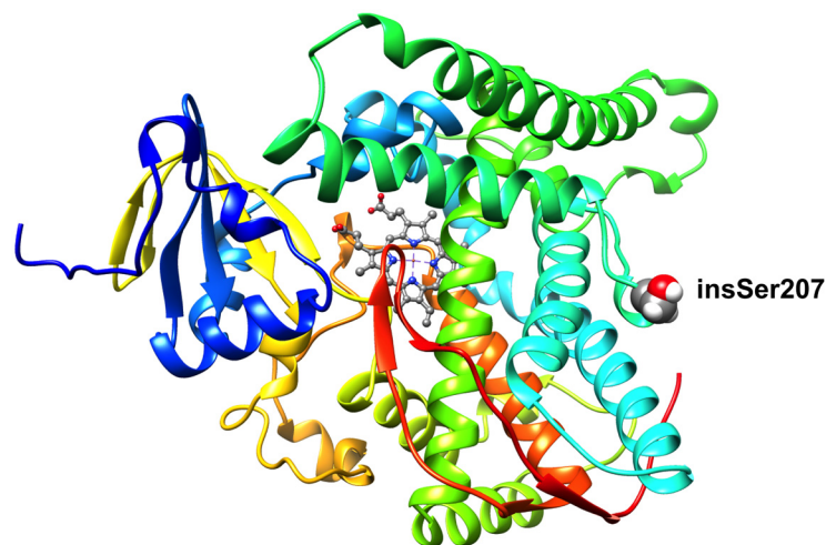
Fig 6. Structural model of human CYP4B1 with insSer207 located in a loop region from G198 to S210. Cartoon representation of the structure of human CYP4B1. The side chain of insSer207 and the heme prosthetic group are shown as spacefilling and ball and stick representations, respectively. Carbon atoms are colored gray, oxygen atoms are colored red, nitrogen atoms are colored blue, and hydrogen atoms are colored white. The figure was generated using UCSF Chimera [43].
