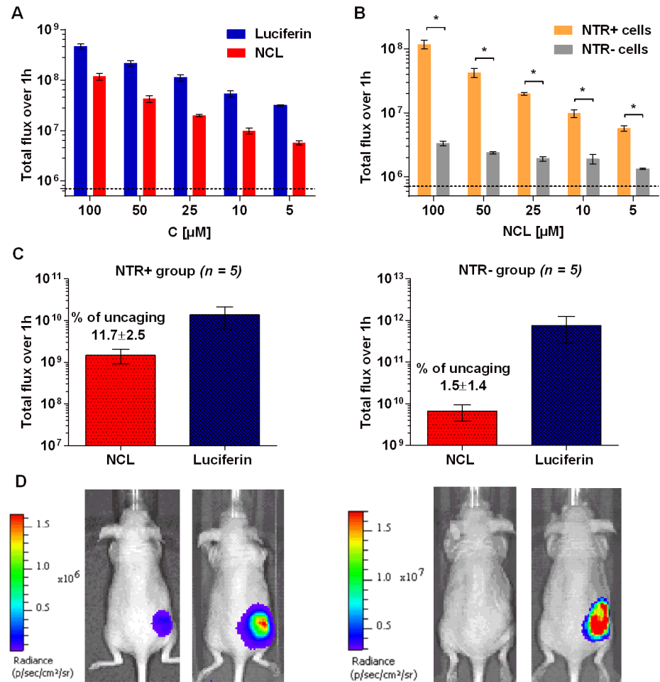
Fig 5. Imaging of NTR activity in cells and in in vivo cancer model with NCL. (A) Concentration-dependent uncaging of NCL in MDA-MB-231 NTR+ luc + cancer cells in comparison with luciferin. (B) Selectivity of NTR imaging by NCL in the same cells in comparison with NTR- luc + cells. The dashed line indicates background (cells only), *P = 0.0001. (C) In vivo imaging of NTR activity in subcutaneous NTR+ and NTR- xenografts (n = 5). Total luminescence over 1 h from IP injection of luciferin (1.5 mg) and NCL (1.9 mg). (d) Representative images of mice 15 min post injection of luciferin or NCL.
