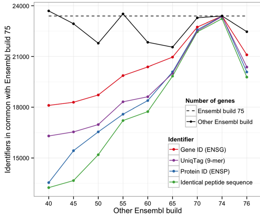
Fig 1. The number of common UniqTag identifiers between build 75 of the Ensembl human genome and nine other builds, the number of common gene and protein identifiers between builds, and the number of genes with peptide sequences that are identical between builds.
