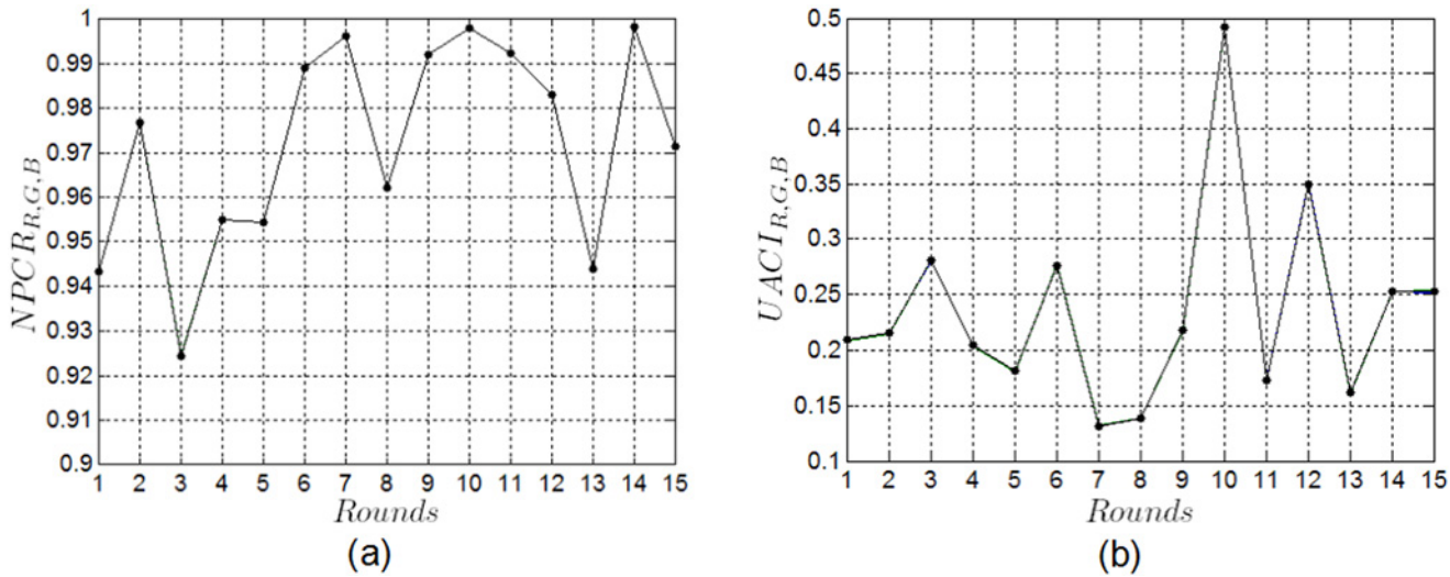
Fig 10. NPCR and UACI performance analysis of the proposed scheme. (a) NPCR versus permutation rounds, (b) UACI versus permutation rounds.
