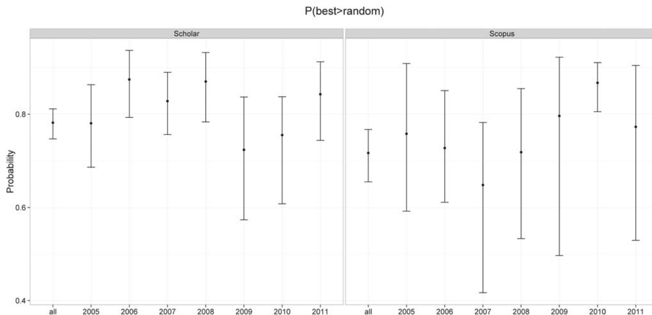
Fig 1. P(\text{best} > \text{random}) for the two datasets analyzed herein. The entry “all” indicates the overall P(\text{best} > \text{random}) . The error bar indicates the 95% confidence interval and the point at the center indicates the mean value of the probability that a best paper will receive more citations than a random non-best paper. The entries 2005 to 2011 indicate the mean and confidence interval of P(\text{best} > \text{random}) for conferences that took place in those years.
