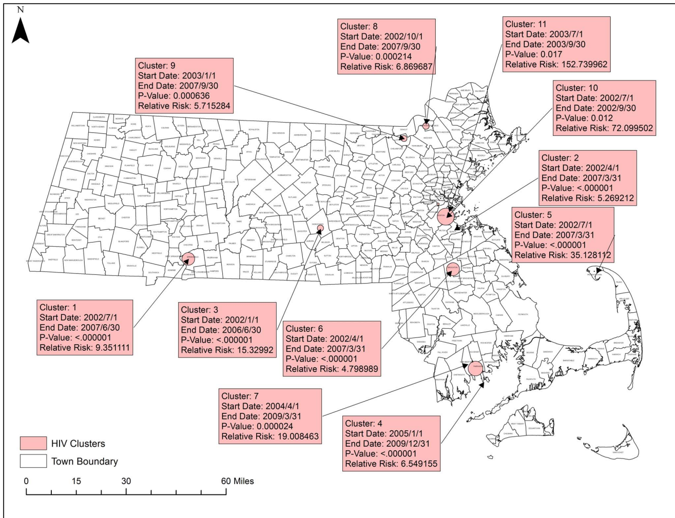
Fig. 11. Statistically Significant Space-time clusters in HIV/AIDS. SatScan was used to test for spatial variation in temporal trends and for significant space-time clusters. Red boxes detail significant space-time clusters. There were no significant spatial variations in temporal trending. Shapefiles were provided by MassGIS, death data were provided by the Massachusetts Department of Public Health, and population estimates were provided by the US Census Bureau. NAD 1983 Massachusetts State Plain was used for projection. Maps created in ArcGIS 10.2.
