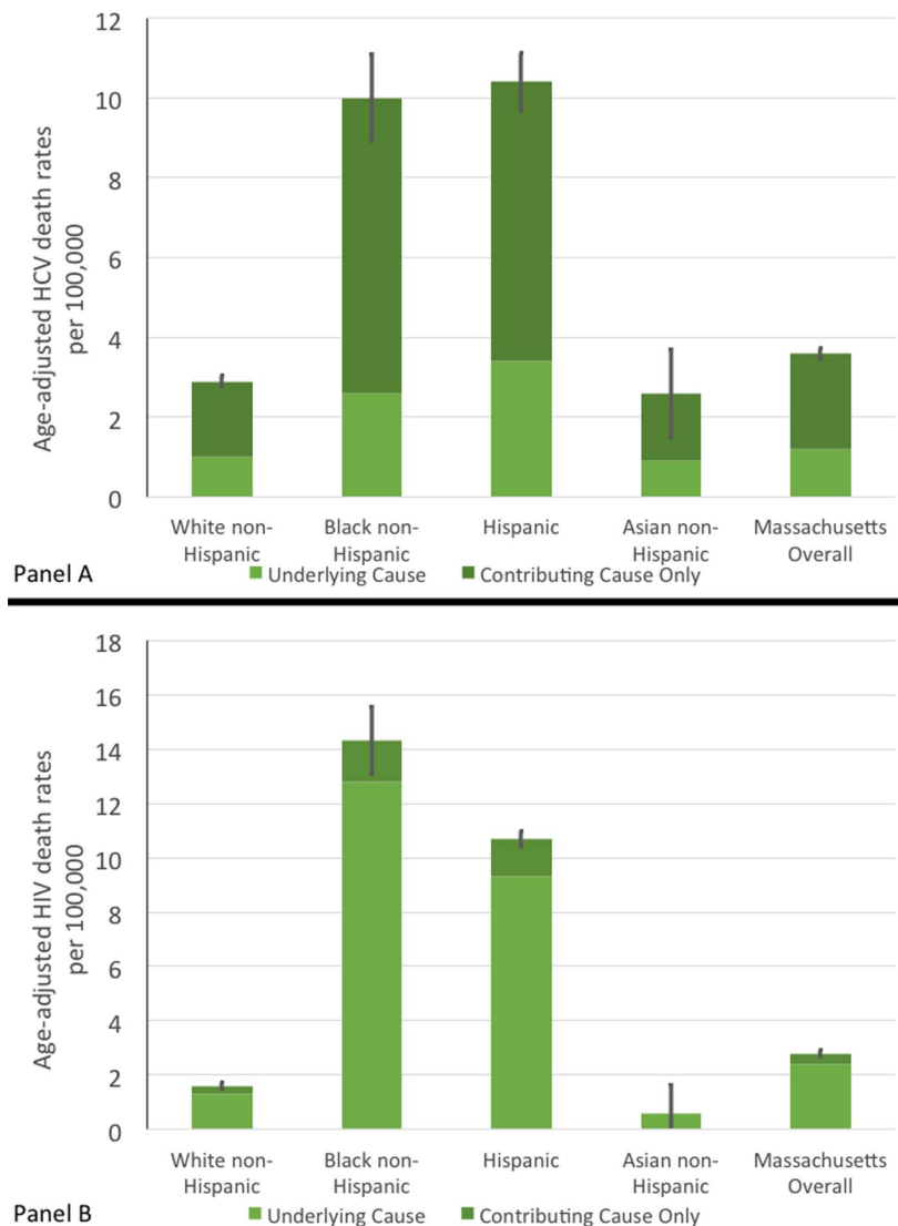
Fig. 3. Standardized HCV and HIV Mortality Rates by Race in MA between 2002–2011. Panel A is Hepatitis C. Panel B is HIV/AIDS.
