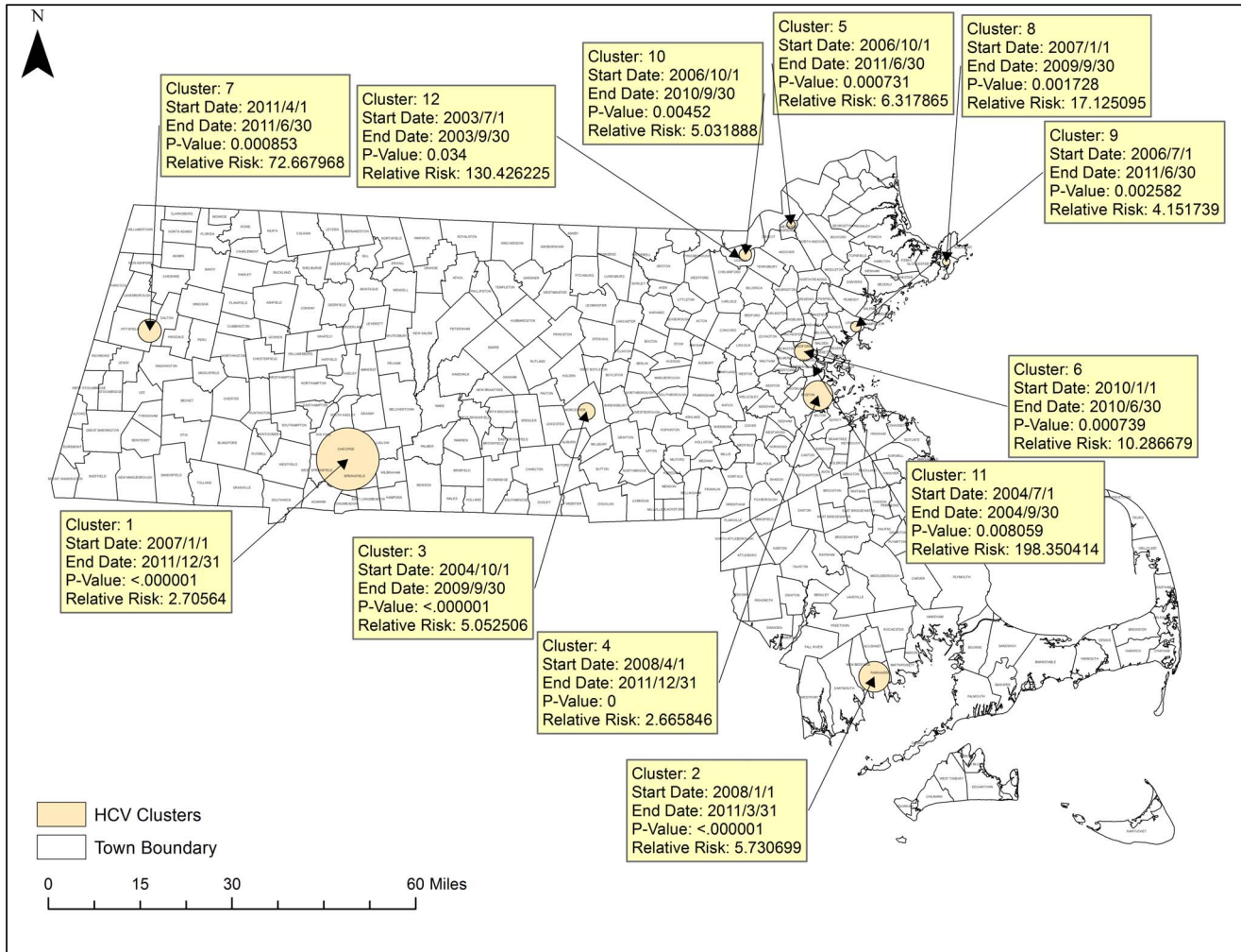
Fig. 10. Statistically Significant Space-time and Spatial Trend Clusters in HCV. SatScan was used to test for spatial variation in temporal trends and for significant space-time clusters. Yellow boxes detail significant space-time clusters. Green boxes detail significant spatial variations in temporal trending. Shapefiles were provided by MassGIS, death data were provided by the Massachusetts Department of Public Health, and population estimates were provided by the US Census Bureau. NAD 1983 Massachusetts State Plain was used for projection. Maps created in ArcGIS 10.2.
