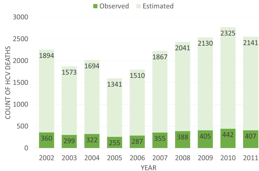
Fig. 2. Observed and Estimated Total HCV Deaths per Year. The observed counts are the totals of both contributing and underlying cause attributed HCV deaths. The estimated is based off the assumption that only 19% of HCV cases are recorded from death certificates and is the estimated total if 100% were to be counted.
