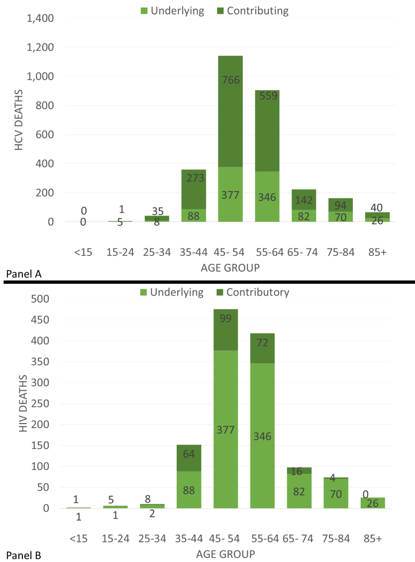
Fig. 4. HCV and HIV/AIDS Deaths by Age in MA between 2002–2011. Panel A is Hepatitis C. Panel B is HIV/AIDS.
