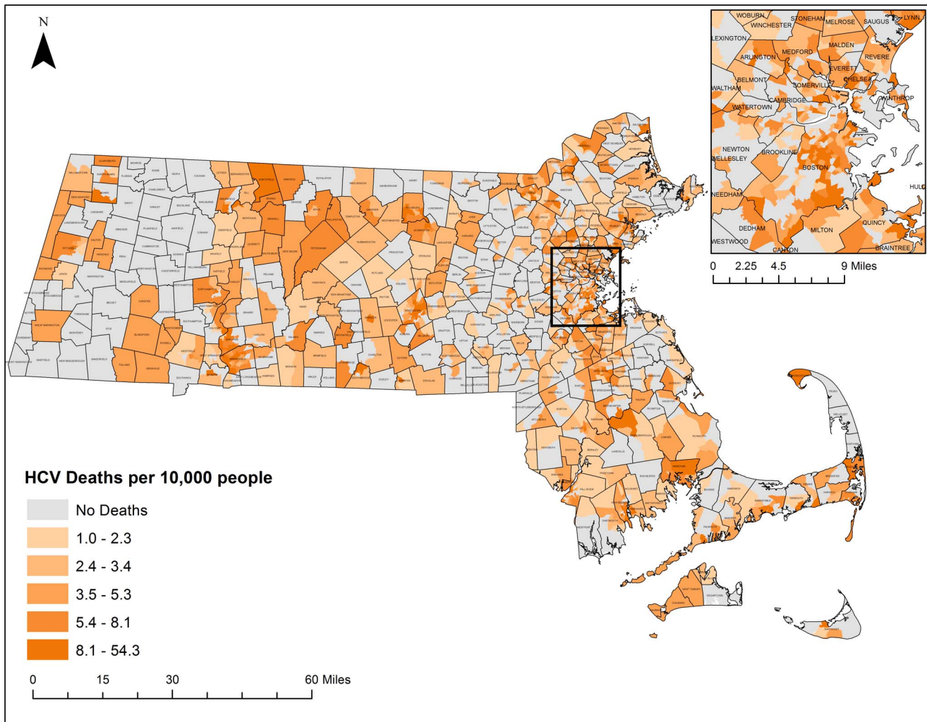
Fig. 6. HCV Mortality rates by census tract, 2002–2011. Crude Mortality Rates were calculated based on the 2010 census population estimates at the census tract level for all-causes of HCV. Rates were classified by quintile. Shapefiles were provided by MassGIS, death data were provided by the Massachusetts Department of Public Health, and population estimates were provided by the US Census Bureau. NAD 1983 Massachusetts State Plain was used for projection. Maps created in ArcGIS 10.2.
