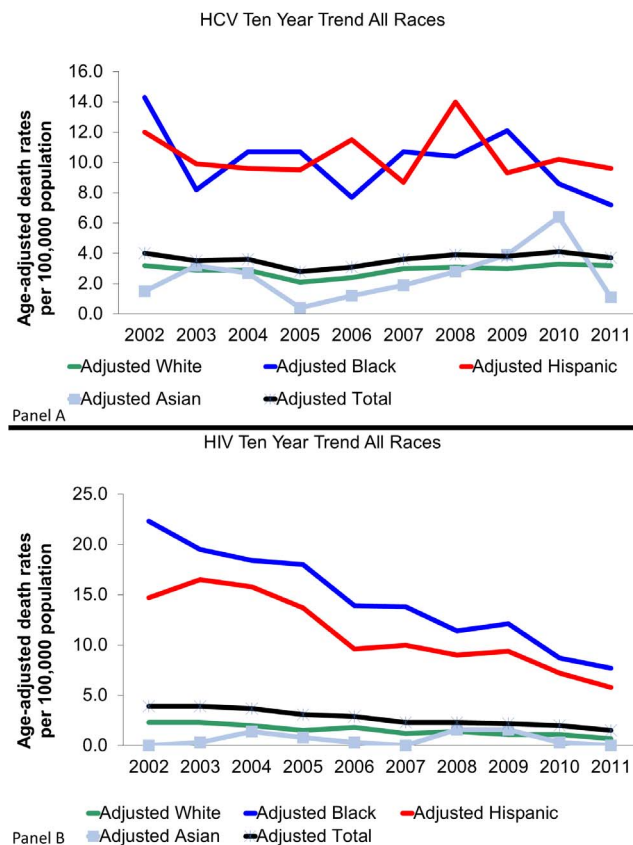
Fig. 5. 10 Year Age Standardized HCV and HIV/AIDS Mortality Trends per 100,000 by Race in MA. Panel A is Hepatitis C. Panel B is HIV/AIDS.
