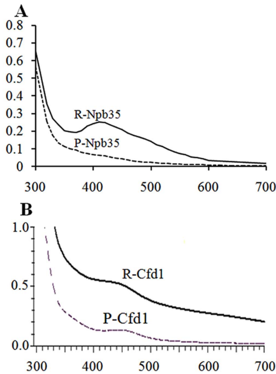
Figure 7. UV-Visible spectra of purified and reconstituted rNbp35 and rCfd1 proteins. A) As purified rNbp-35 and rNbp35 after chemical reconstitution was scanned in the UV-Vis range to detect Fe-S cluster. Solid and dashed lines represent reconstituted Nbp35 and purified Nbp35, respectively. B) UV-visible spectra of purified rCfd1 and reconstituted rCfd1 protein in which, solid and dashed lines represent reconstituted rCfd1 and purified rCfd1, respectively. doi:10.1371/journal.pone.0108971.g007
