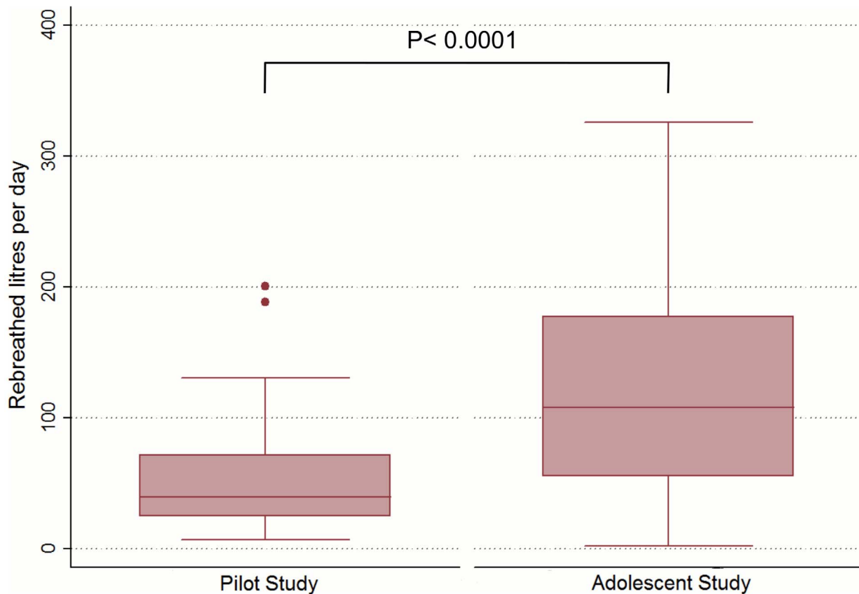
Figure 2. Daily volumes of rebreathed air in the pilot study and the adolescent study. Pilot study (left bar) shows median, inter-quartile ranges and maximum and minimum daily volumes of rebreathed air from others for 17 adults providing 29 daily records. Adolescent study (right bar) shows median, inter-quartile ranges and maximum and minimum daily volumes of rebreathed air of 108 daily records from 63 adolescents living in a high TB prevalence township. N.B. A single outlier value of 550 litres per day for the adolescent study is not shown as it exceeds the maximal value of the ordinate scale.
