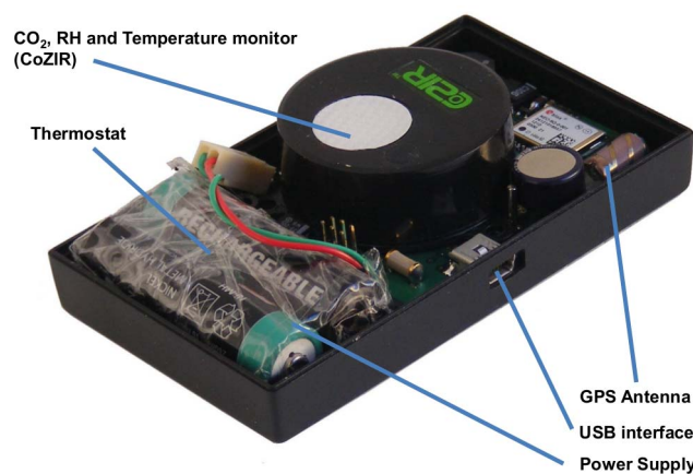
Figure 1. Portable logger to measure CO 2 concentration, temperature and humidity. An internal view of the portable personal CO 2 logger incorporated a COZIR Ambient 0–1% transducer (Gas Sensing Solutions Ltd., Glasgow, United Kingdom), GPS sensor, independent power supply and USB interface. Unit dimensions were length 10 cm, width 6 cm and depth 2.5 cm. doi:10.1371/journal.pone.0106622.g001
