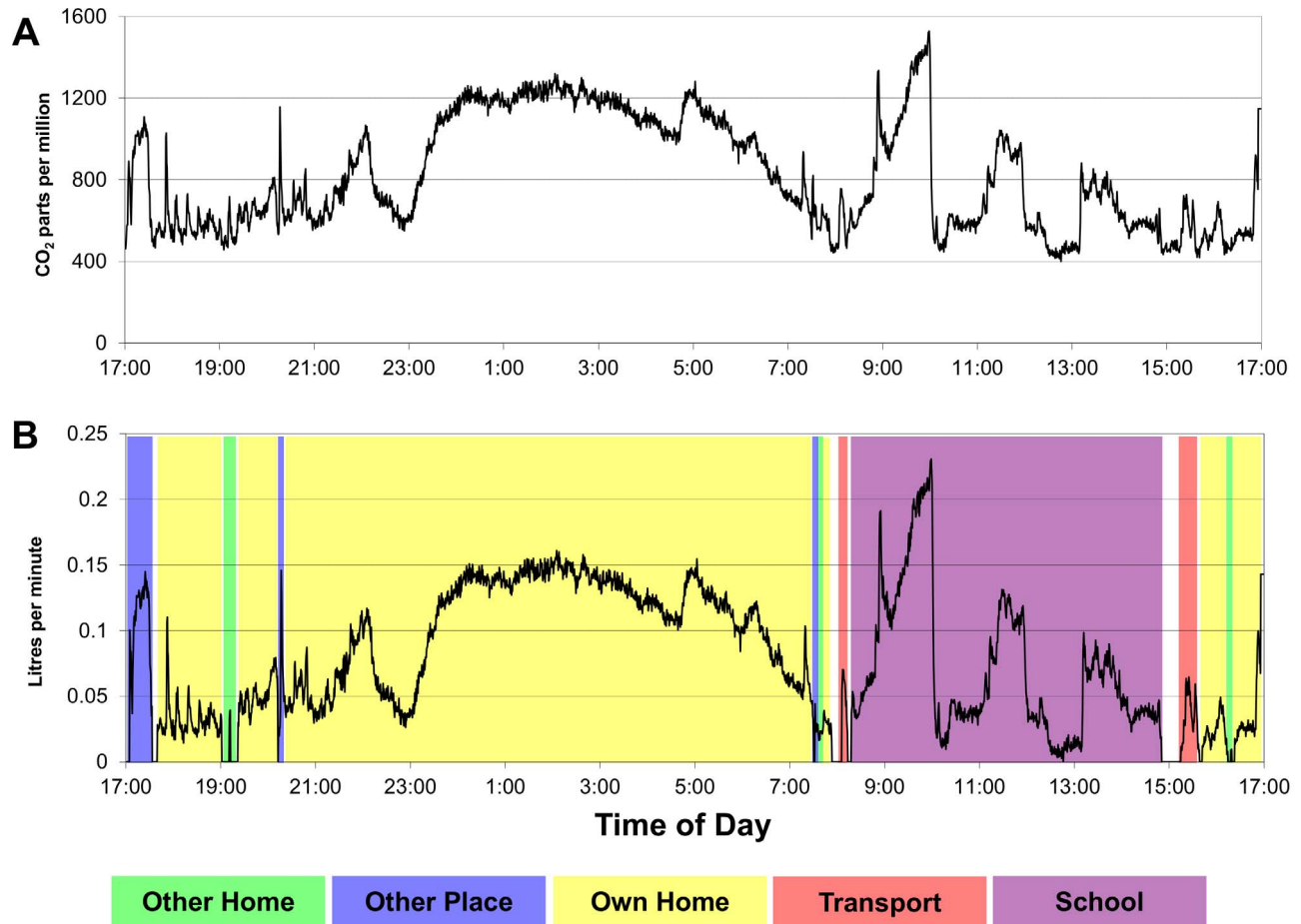
Figure 3. Figure 3 A: Ambient parts per million of CO 2 recorded at minute intervals by the logging device carried by a subject during a 24-hour period. Figure 3 B: Litres per minute of rebreathed air with additional allocation to specific locations. Litres per minute of rebreathed air were calculated for a 24-hour period (transformation from ambient CO 2 levels in Figure 2A) and additionally allocated to specific locations using diary and GPS information. The volume of rebreathed shared air is represented by the area under the curve for each location visited and the daily rebreathed volume is the sum of all volumes at all locations visited. doi:10.1371/journal.pone.0106622.g003
