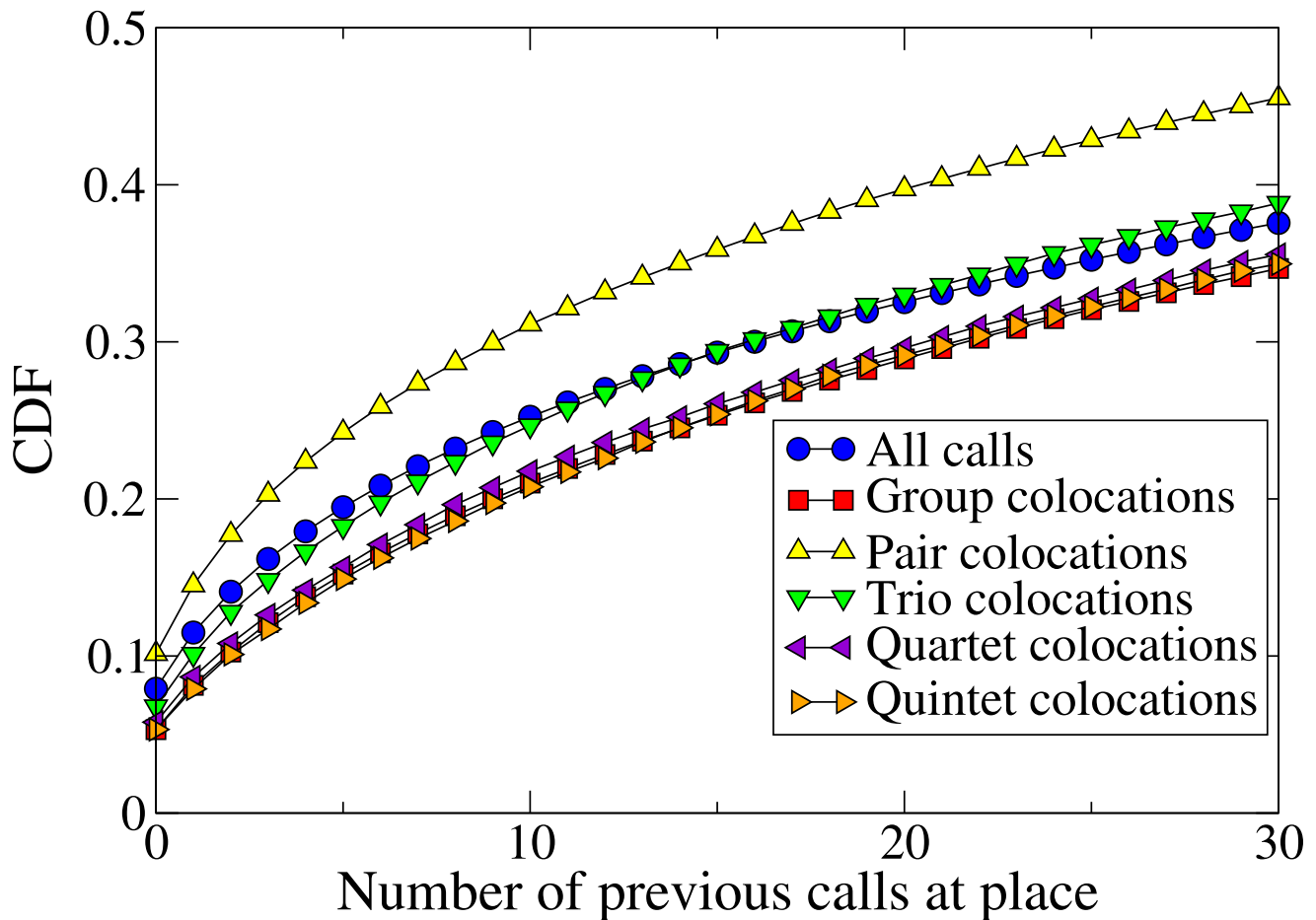
Figure 7. Cumulative distribution function (CDF) of the number of previous calls made or received by a cellphone user at a location, for collocated groups of various sizes. Pairs are more likely to meet at new places, in agreement with the Foursquare data, but bigger groups than this tend to meet at familiar locations. doi:10.1371/journal.pone.0105816.g007
