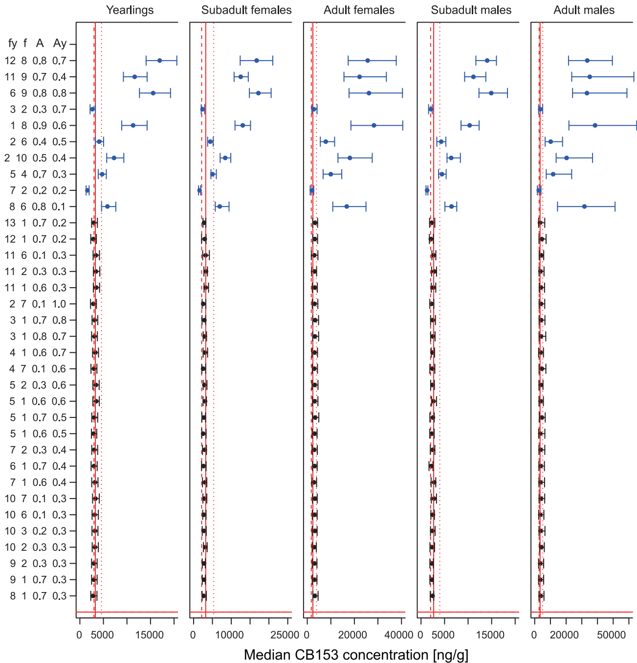
Figure 4. Medians of CB153 concentration of bear sub groups. Comparison between median observed CB153 concentrations in East Greenland polar bears (solid red lines) and CB153 concentration simulated using the best-fitting parameter combinations (black) or randomly selected parameter combinations (blue). Quartiles are shown as bars for model predictions and as dashed red lines for East Greenland bears. doi:10.1371/journal.pone.0104037.g004
