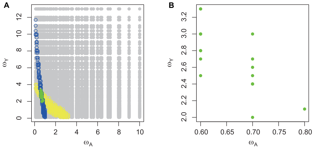
Figure 3. Tested combinations of deposition efficiencies and field metabolic factors. a) Only few combinations of proportionality constants: \omega_A (=A_A \times f_A) and \omega_Y (=A_Y \times f_Y) produced predictions not significantly different from actual data: in older bears (blue), yearlings (yellow) or both groups (green). All tested combinations are coloured grey. b) Combinations of \omega_A and \omega_Y that produced predictions not significantly different from actual data in both studied groups exhibited a negative relationship. doi:10.1371/journal.pone.0104037.g003
