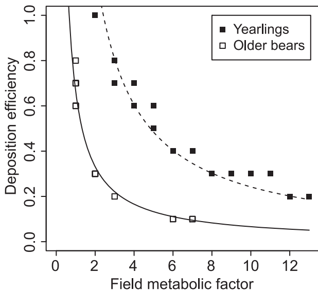
Figure 2. Relationship between deposition efficiency and field metabolic factor. Within the parameter combinations that produced matching predictions the deposition efficiency was inversely proportional to the field metabolic factor in both groups; the yearlings and older bears. Solid curve: A_A = 0.6626/f_A , dashed curve: A_Y = 2.42/f_Y . doi:10.1371/journal.pone.0104037.g002
