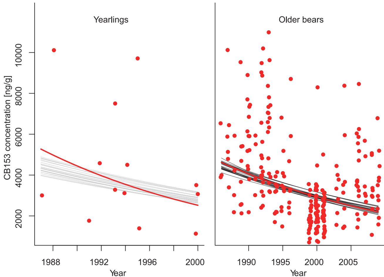
Figure 1. Time trend in polar bear CB153 concentrations. Red dots show the CB153 concentrations in individual East Greenland bears across the study period. Red curve shows log – linear trend in the data. Grey and black curves show simulated trends in CB153 concentrations produced using parameter combinations that produced predictions that did not differ from the observed trends in East Greenland for yearlings and older bears, respectively.
