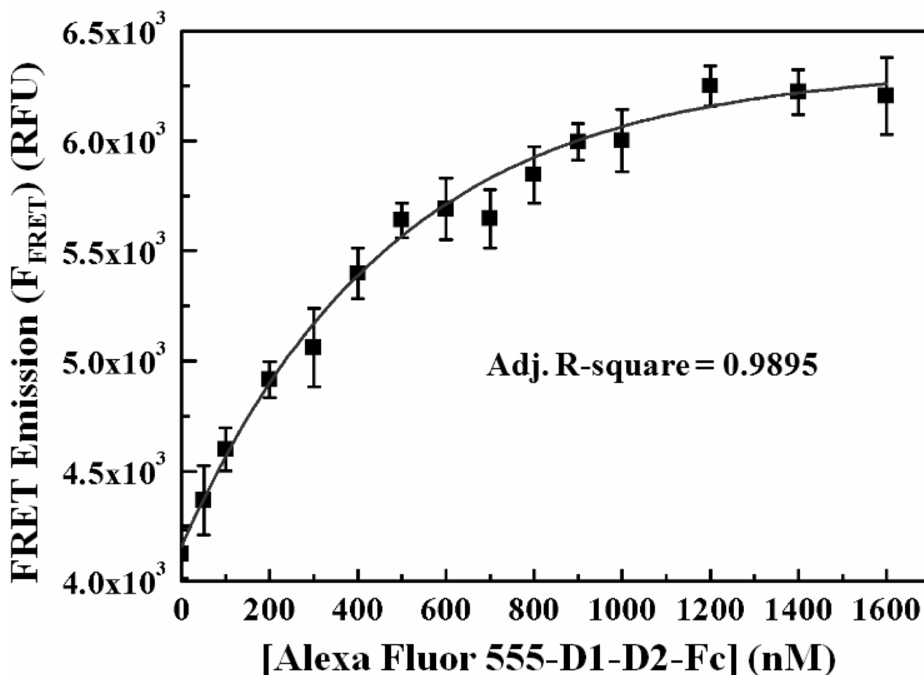
Figure 5. Determination of dissociation constant ( K_d ) and maximum FRET emissions ( F_{\text{FRETmax}} ) signal. The plot shows the fitting curve of FRET emission signal with equation (6). The F_{\text{FRETmax}} and the corresponding K_d of the LFA-1/D1-D2-Fc interaction were determined to be 6.33 \times 10^3 RFU and 17.93 \pm 1.34 nM, respectively. The flattening of the FRET emission signal, when the acceptor concentration exceeds \sim 500 nM, can be attributed to the fact that the increased acceptor concentration gradually saturates the number of donor binding pairs. doi:10.1371/journal.pone.0102572.g005
