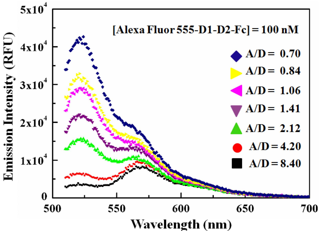
Figure 6. Determination of A/D ratio for optimal FRET between Alexa Fluor 488-LFA-1 and Alexa Fluor 555-D1-D2-Fc. Fluorescence emission scans were obtained for the Alexa Fluor 488-LFA-1 and Alexa Fluor 555-D1-D2-Fc mixture, where the concentration of Alexa Fluor 555-D1-D2-Fc was kept constant at 100 nM and that of Alexa Fluor 488-LFA-1 was varied: 25 nM (A/D=8.40), 50 nM (A/D=4.20), 100 nM (A/D=2.12), 150 nM (A/D=1.41), 200 nM (A/D=1.06), 250 nM (A/D=0.84) and 300 nM (A/D=0.70). The mixtures were excited at 470 nm. The highest FRET efficiency (~53.51%) was obtained for A/D=2.12. For both 4.20 and 8.40 A/D ratios, the donor peak intensity is very small compared to the acceptor peak. These higher emission counts at 4.20 and 8.40 A/D can be attributed to the direct emission of the acceptor as the acceptor concentration exceeds the saturating concentration required to saturate the donor binding pairs. doi:10.1371/journal.pone.0102572.g006
