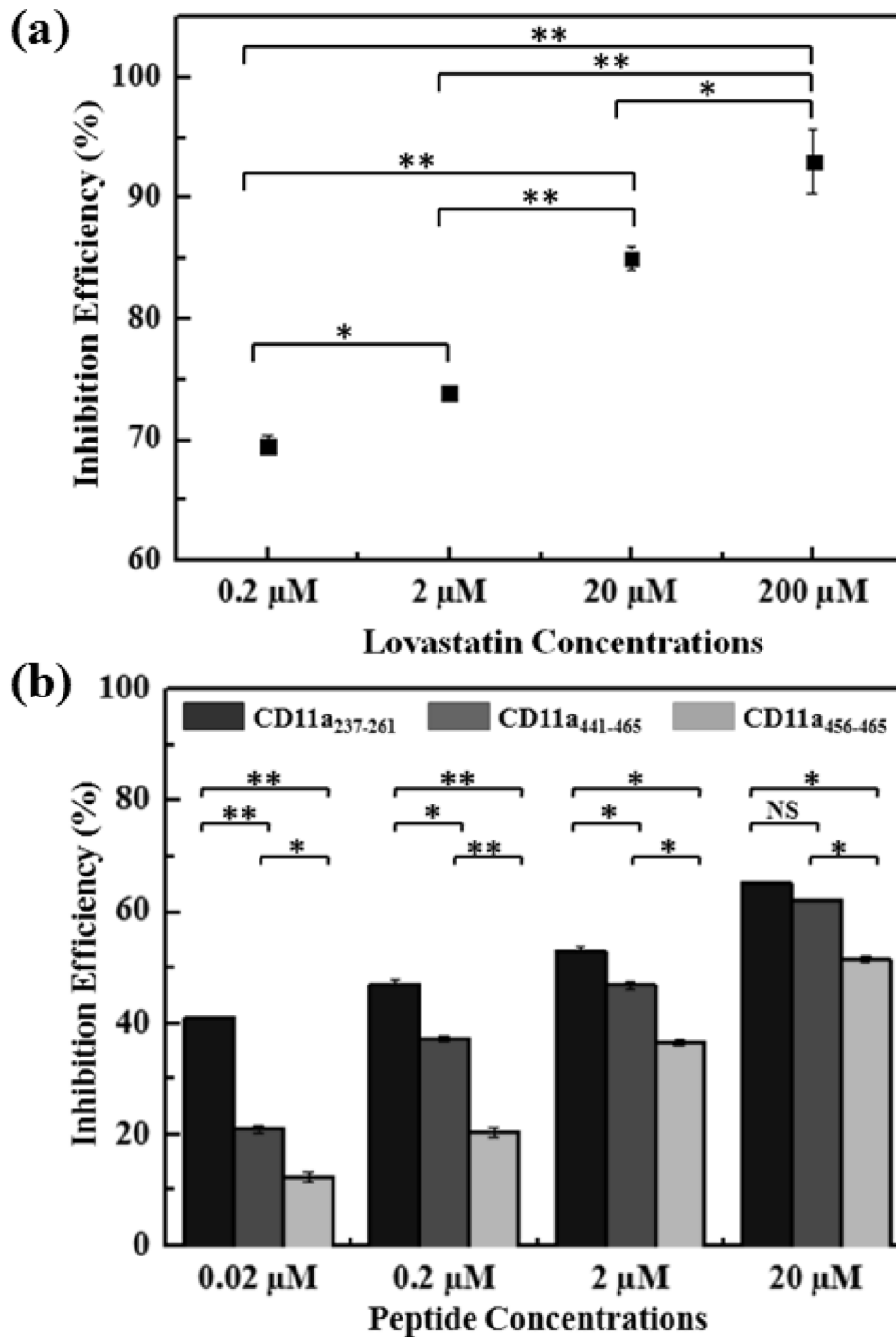
Figure 7. A summary of the inhibitory effects (to the LFA-1/ICAM-1 interactions) of (a) lovastatin; and (b) LFA-1 derived peptides. “*” and “**” denote statistical significance with p < 0.05 and p < 0.005 , respectively, from student t-test. NS: Not Significant. In (a), different concentrations of lovastatin were added to the FRET mixture of Alexa Fluor 488- LFA-1 (100 nM) and Alexa Fluor 555-D1-D2-Fc (100 nM). The inhibition efficiency of lovastatin increased from 69.48 \pm 0.77\% at 0.2 \mu\text{M} to 90.03 \pm 0.06\% at 200 \mu\text{M} . This result confirms that this FRET based screening assay is capable of identifying/classifying inhibitors of the LFA-1/ICAM-1 interaction based on inhibition efficiency study. From (b), a comparison of the inhibition efficiencies (to the LFA-1/ICAM-1 interactions) of three LFA-1 derived peptides CD11a 237-261 , CD11a 441-465 , and CD11a 456-465 indicates that CD11a 237-261 exhibits the highest inhibition efficiency while CD11a 456-465 the lowest for all the concentrations tested in this study.
