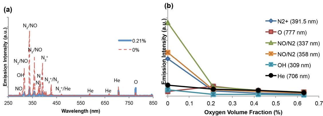
Figure 8. (a) Comparison between spectrum of He/O 2 mixture plasma jet and He plasma jet at output voltage 3.16 kV. (b) The trend of major plasma generated RNS and ROS with oxygen volume fraction change at 0, 0.21, 0.42, 0.63%. doi:10.1371/journal.pone.0098652.g008
