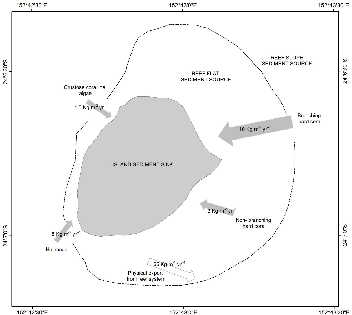
Figure 2. Conceptual model of the carbonate budget for Lady Elliot Island.
