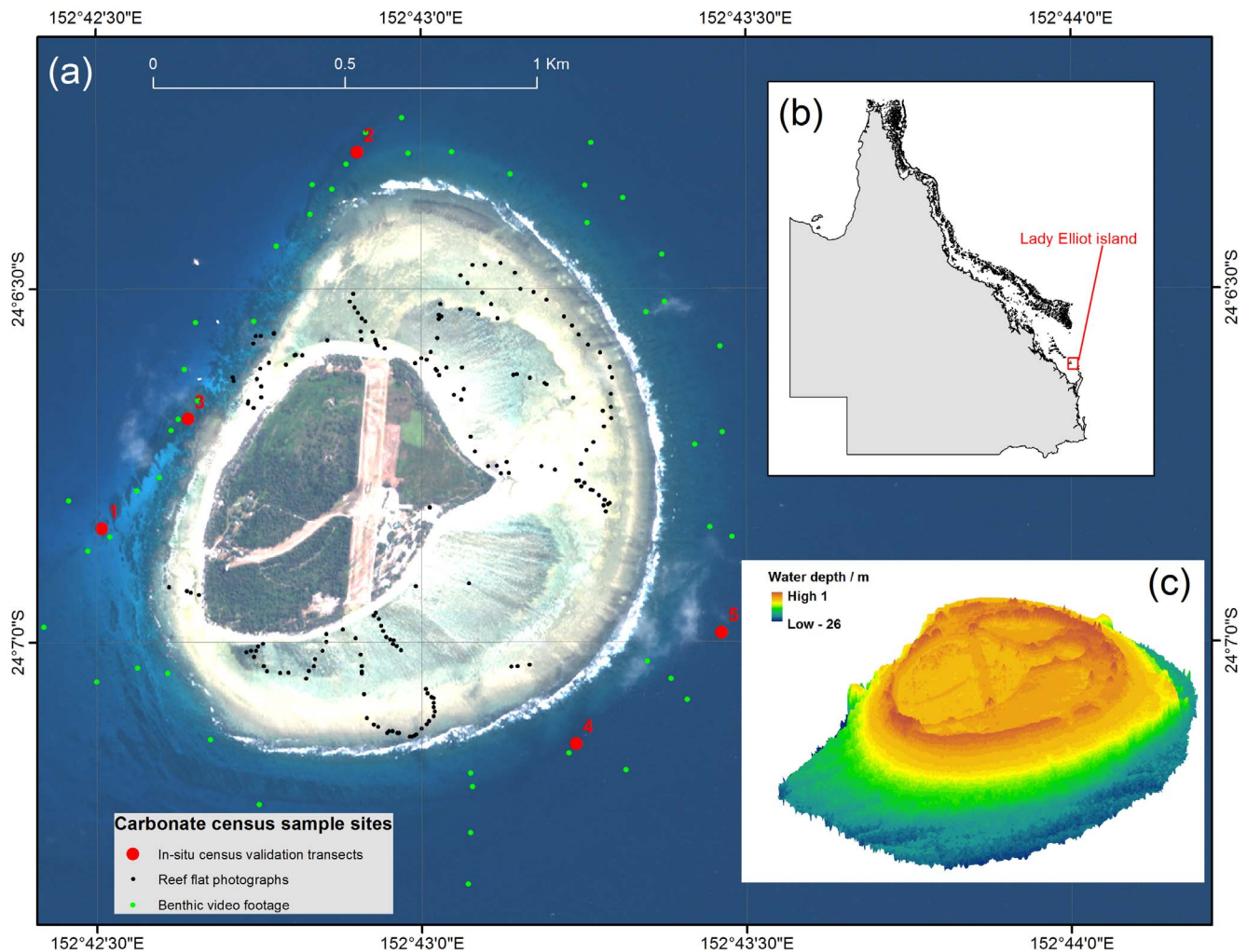
Figure 1. Fieldwork undertaken at Lady Elliot Island, Great Barrier Reef (24°07'S:152°43'E). (a) A Quickbird satellite image of Lady Elliot Island, showing sample sites for the carbonate production census (red dots, numbering relates to sites detailed in Table 2), reef flat and reef slope ground referencing points (black and green dots) (b) The location of Lady Elliot Island along the Queensland coastline, at the southern end of the Great Barrier Reef, (c) a digital elevation model of Lady Elliot island and the surrounding reef platform. doi:10.1371/journal.pone.0094067.g001
