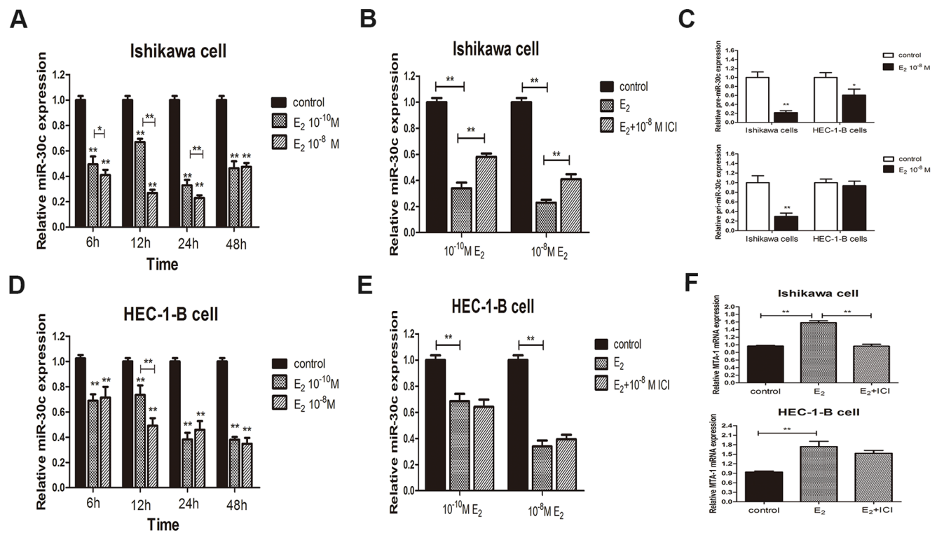
Figure 5. Estrogen regulates the expression of miR-30c in EC cells. (A). MiR-30c was decreased upon treatment with 10^{-8} M and 10^{-10} M E_2 at 6, 12, 24 and 48 h after treatment by qRT-PCR analysis in Ishikawa cells. The treatment with 10^{-8} M E_2 exerted a more significant inhibition except at 48 h. (B). 10^{-8} M ICI182780 partially reversed the reduction of miR-30c levels induced by the treatment with 10^{-8} M and 10^{-10} M E_2 at 24 h after cotreatment in Ishikawa cells. (C). Pre-miR-30c levels were reduced by E_2 treatment in both the Ishikawa and HEC-1-B cells (upper). Pri-miR-30c levels were reduced by E_2 treatment in Ishikawa but not in HEC-1-B cells (lower). (D). MiR-30c levels were reduced upon 10^{-8} M and 10^{-10} M E_2 treatment at 6, 12, 24 and 48 h after treatment by qRT-PCR analysis in HEC-1-B cells. The effect of the two concentrations differed at 12 h after treatment. (E). 10^{-8} M ICI182780 did not reverse reduction of miR-30c levels induced by the treatment with 10^{-8} M and 10^{-10} M E_2 at 48 h after cotreatment in HEC-1-B cells. (F). Treatment with 10^{-8} M E_2 up-regulated mRNA expression of MTA-1 in both the Ishikawa cells and HEC-1 cells at 24 and 48 h, respectively, an effect that was reversed by cotreatment with 10^{-8} M ICI182780 in the Ishikawa cells (upper) but not the HEC-1-B cells (lower). (* P < 0.05 , ** P < 0.01 ).
