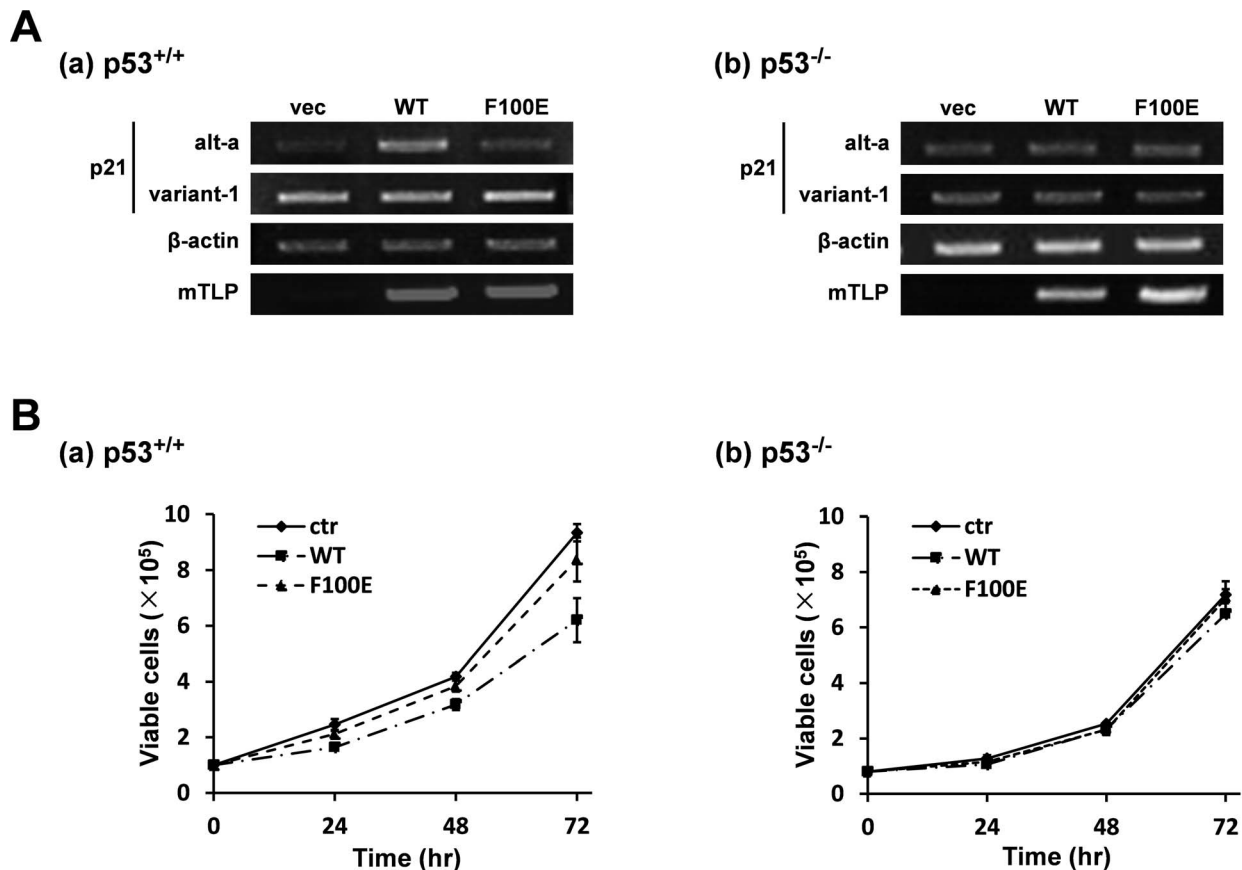
Figure 7. Effect of F100E mutation of TLP on the expression of endogenous p21 gene and cell growth. (A) Wild-type (a) and p53 -/- cells (b) were transfected with expression vectors of wild-type and mutant (F100E) TLPs, and two species of p21 transcripts were determined by RT-PCR as described in a legend of Fig. 4. (B) Wild-type and mutant TLP-transfected native (a) and p53 -/- (b) cells were cultured for 24 hr. Cells (1 × 10 5 ) were replated and cell numbers were counted every 24 hr. ctr: vacant plasmid. doi:10.1371/journal.pone.0090190.g007
