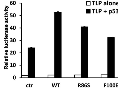
Figure 6. Examination of mutant TLPs on transcriptional activation and p53 binding. (A) Structural relationship between TBP and TLP. Amino acid numbers are indicated from N-termini. TLP covers the evolutionarily conserved region of TBP. A putative p53-binding region in TBP deduced from deletion analyses [44] and its TLP counterpart (from 63 to 115) are depicted as a gray area. Positions of AAs of the TLP mutants used in this study (R86S, F100E, and F114E) are indicated with vertical arrowheads. (B) Transcription activation function of wild-type (WT) and mutant TLPs were assayed in native (a) and p53 -/- (b) cells. (C) Binding of TLP and p53. Wild-type and F100E TLPs were analyzed for the p53-binding ability by two-hybrid assay.
