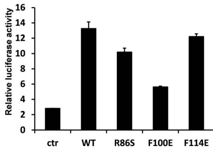
Figure 6. Examination of mutant TLPs on transcriptional activation and p53 binding. (A) Structural relationship between TBP and TLP. Amino acid numbers are indicated from N-termini. TLP covers the evolutionarily conserved region of TBP. A putative p53-binding region in TBP deduced from deletion analyses [44] and its TLP counterpart (from 63 to 115) are depicted as a gray area. Positions of AAs of the TLP mutants used in this study (R86S, F100E, and F114E) are indicated with vertical arrowheads. (B) Transcription activation function of wild-type (WT) and mutant TLPs were assayed in native (a) and p53 -/- (b) cells. (C) Binding of TLP and p53. Wild-type and F100E TLPs were analyzed for the p53-binding ability by two-hybrid assay.
