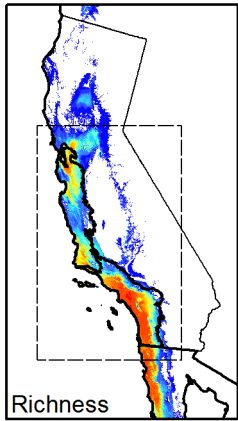
Current Worldclim (1950-2000)
