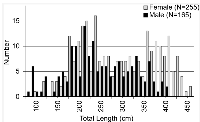
Figure 1. Size distribution of male and female tiger sharks captured in Hawaii 1993–2013. doi:10.1371/journal.pone.0084799.g001
