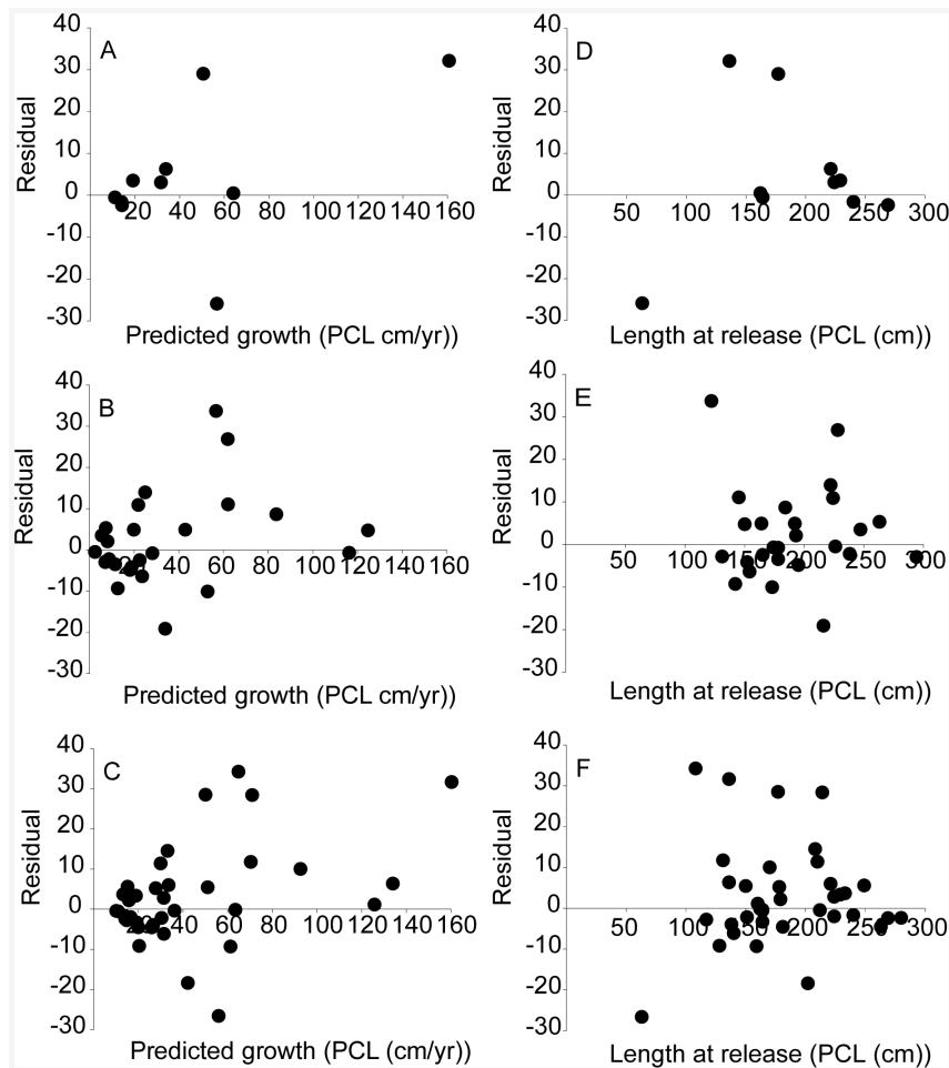
Figure 2. Francis growth model residual plots. Plots of Francis growth model residuals (observed minus predicted) versus predicted growth (PCL (cm/yr)) for tiger shark a) male, b) female, and c) sexes combined and length-at-release (PCL (cm)) for d) male, e) female, and f) sexes combined. doi:10.1371/journal.pone.0084799.g002
