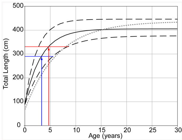
Figure 3. Von Bertalanffy growth curves for Hawaii tiger sharks (both sexes combined). Growth curves are derived from parameters generated by the best fit GROTAG model (Solid line = average growth. Dashed line = upper and lower 95% growth estimates) and analysis of vertebral rings (De Crosta et al. [16], dotted grey line). Arrows indicate estimates of minimum age at maturity for male (blue) and female (red) tiger sharks based on size at maturity estimates (horizontal lines) provided by Whitney and Crow (2007) [7]. doi:10.1371/journal.pone.0084799.g003
