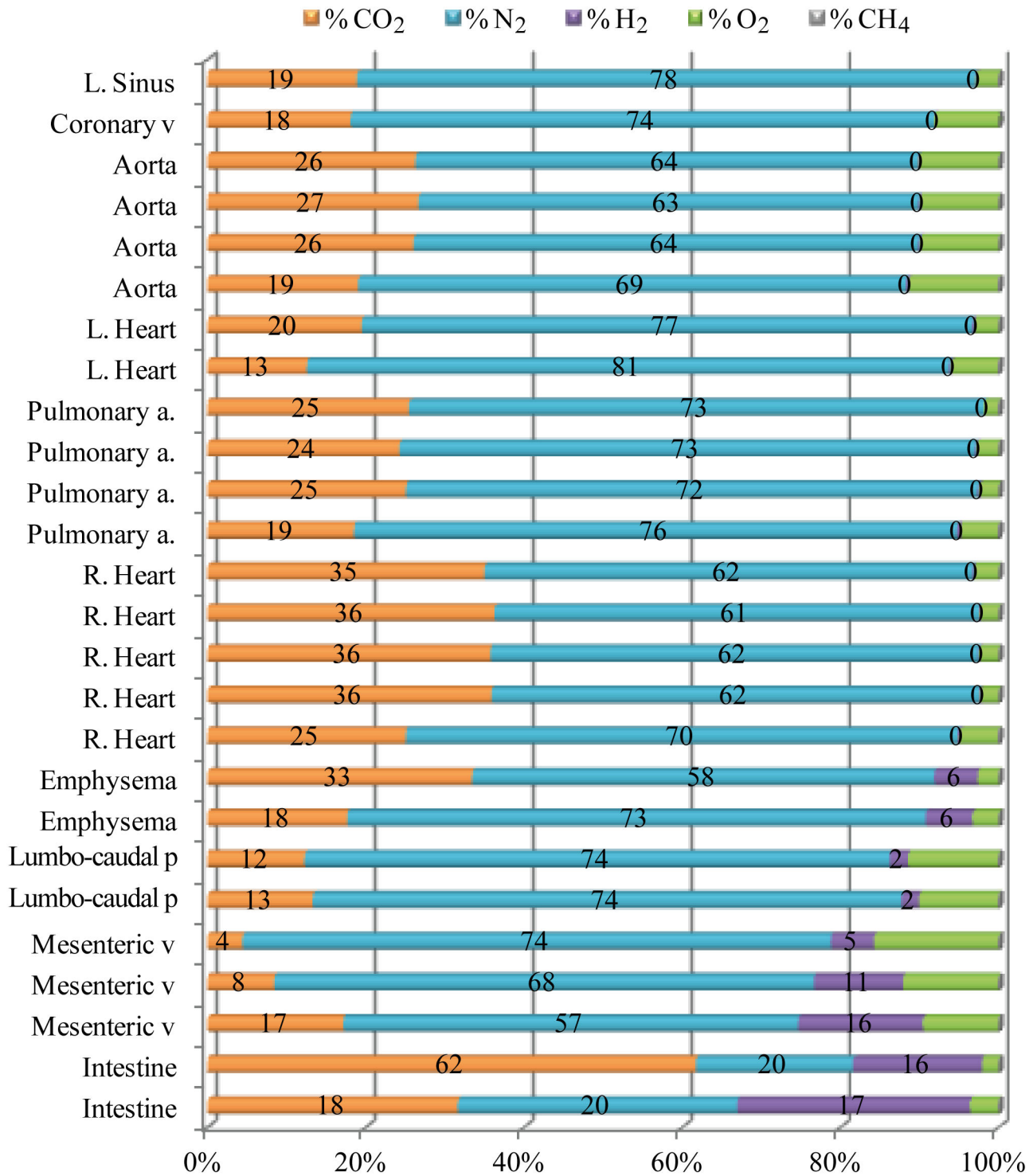
Figure 4. Gas composition of the bubbles found in D06200. Relative gas composition (% μmol) of samples taken at different body locations of D06200, a bycaught short beaked common dolphin. Necropsy was performed within 12 h post mortem. Abbreviations: L, left; R, right; v, vein; a, artery; p, plexus.
