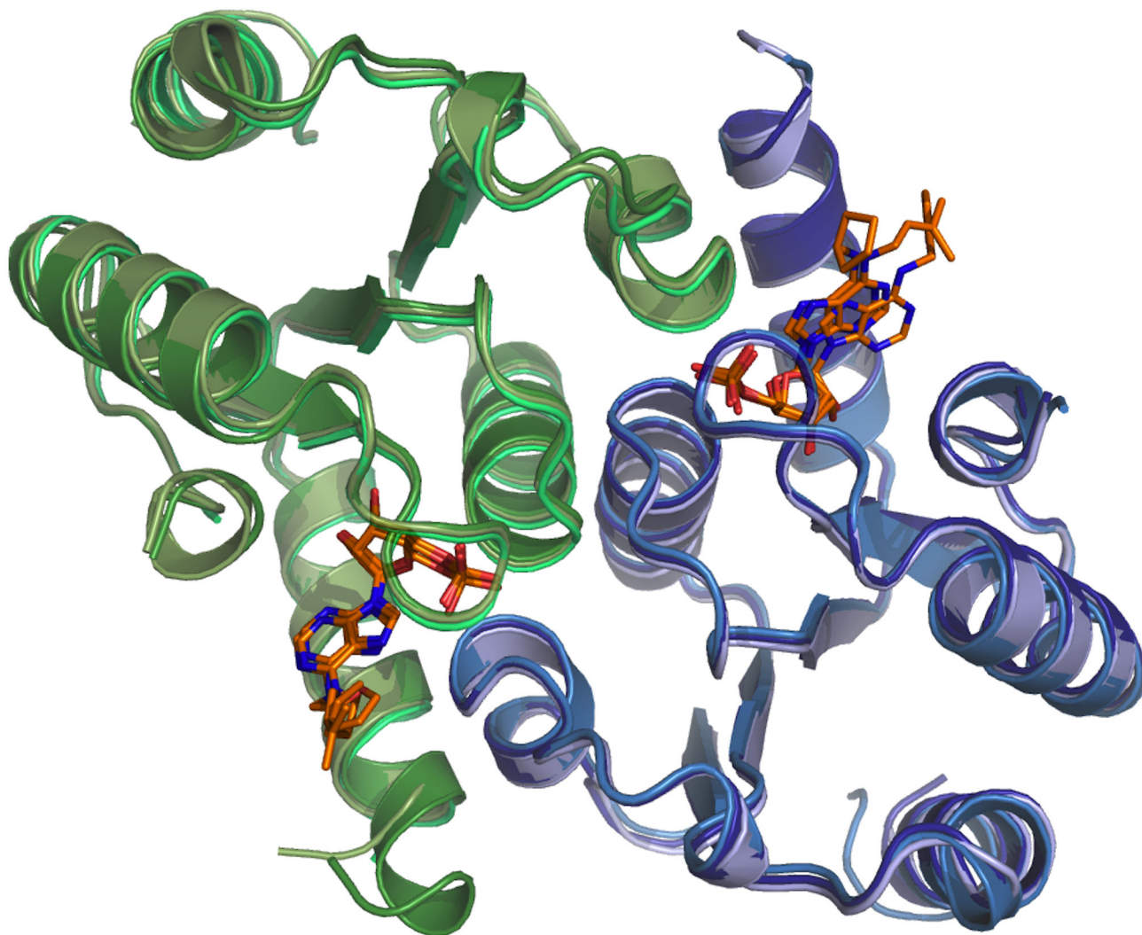
Figure 5. Superposed crystal structure of rat DNP1 in complex with nucleotides N^6 -cyclopentyl AMP, N^6 -furfuryl AMP and N^6 -isopentenyl AMP (compounds numbered 7, 5 and 1 in the text, respectively). One dimer of each complex is shown in blue/green ribbons. The corresponding ligands are shown as orange sticks. The figures were generated by Pymol ( www.pymol.org ).
